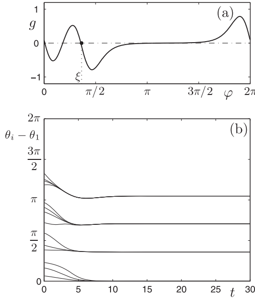
Fig. 3. Panel (a) shows the coupling function (3.14, 3.15) for \xi = 2\pi/(M + 1.5) and M = 4 . This function also supports stable 4-cluster states. The corresponding time series are shown in panel (b) for N = 15 coupled oscillators; each curve corresponds to a particular \theta_i - \theta_1 for i = 1, \dots, 15 .
