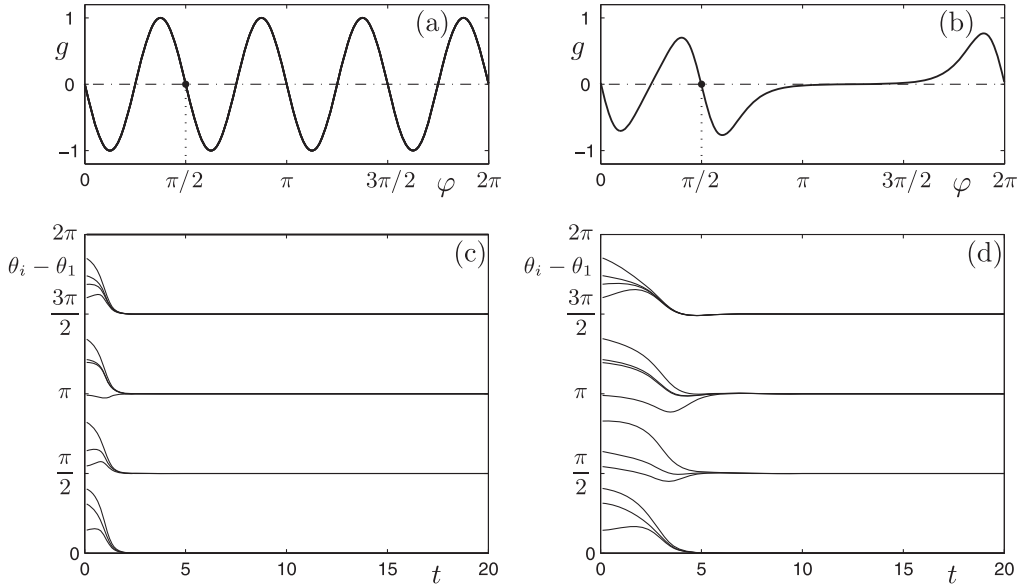
Fig. 2. The coupling functions (3.3) and (3.14, 3.15) are displayed in panels (a) and (b), respectively, for M = 4 and \xi = 2\pi/M . They both support stable 4-cluster states. Panels (c) and (d) show the corresponding time series of phases for a system of N = 15 coupled oscillators. Each curve corresponds to a particular phase difference \theta_i - \theta_1 for i = 1, \dots, 15 . Observe that the convergence is slower in case (d) suggesting that the tangential and transverse eigenvalues are closer to the imaginary axis.
