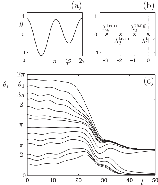
Fig. 1. Designing coupling function for stable 2-cluster partitions with cluster sizes a_1 = 6 and a_2 = 9 for N = 15 oscillators. The phase difference between the clusters is set to \pi/2 . The designed coupling function (2.34) with L = 2 and Fourier coefficients u_1 = 1/36 , v_1 = -61/180 , u_2 = 5/6 , v_2 = 13/360 is shown in panel (a) and the corresponding eigenvalues are displayed in panel (b). The numerical simulation results are shown in panel (c) where each curve corresponds to a particular phase difference \theta_i - \theta_1 for i = 1, \dots, 15 . Observe that the system converges to the designed 2-cluster partition (2.37).
