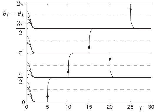
Fig. 4. Realizing the ‘abacus dynamics’ by transferring oscillators between M = 4 clusters for N = 15 oscillators. The same coupling function and initial conditions are used as in Fig. 2(c). The discrete path (3.16) is realized by resetting the phases of individual oscillators by \pm 1 at t = 5, 10, 15, 20, 25 . The horizontal dashed lines show the locations of unstable clusters: the applied resets must exceed the distance \pi/4 between stable and unstable clusters to lead to transitions.
