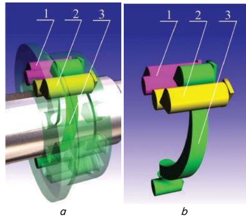
Fig. 9. Flow-through parts of distributor: a – channels; b – images of flow-through parts; 1 – channel, shown in Fig. 7, b; 2 – channel, shown in Fig. 7, c; 3 – channel, shown in Fig. 7, d
