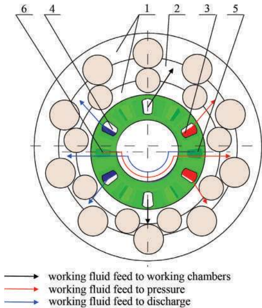
Fig. 5. Schematic of the working fluid feed to the working chambers of a hydraulic motor: 1 – tooth gear couple; 2 – working chambers formed by the toothed gearing; 3 – overlapping of the injection windows of control valve with the working windows of distributor; 4 – overlapping of the discharge windows of control valve with the working windows of distributor; 5 – overlapping of the discharge windows of control valve with the discharge windows of distributor; 6 – overlapping of the injection windows of control valve with the discharge windows of distributor
