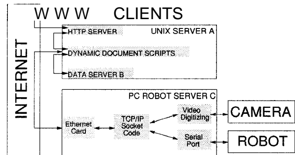
Figure 4: System Architecture
