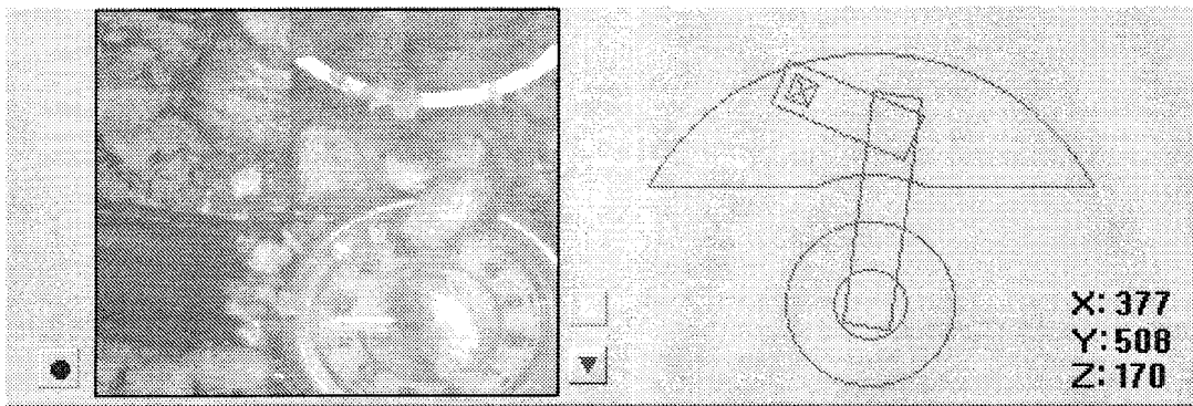
Figure 3: The "status image". At the right is a schematic top view of the semi-annular workspace and robot linkage. At left is a CCD camera image of the view directly beneath the robot end-effector. UpPown buttons are included for Z motion of the camera, and the round button is used to blow a burst of compressed air into the sand.
