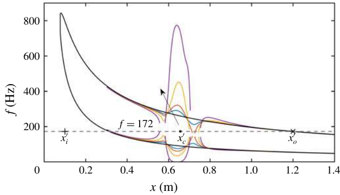
FIGURE 2. (Colour online) Positions of the inlet x'_i (+) and indentation centre x'_c (●) and the outlet x'_o (×). The horizontal dashed line indicates the physical frequency at which experiments are conducted. The solid dark line indicates the neutral stability curve of the flat-plate boundary layer. The modified neutral stability curves are shown by the coloured lines for 2-D base flows computed for the case \lambda = 162 mm; arrow indicates the direction of increasing depth h = 0.18, 0.36, 0.81, 2.17 mm.
