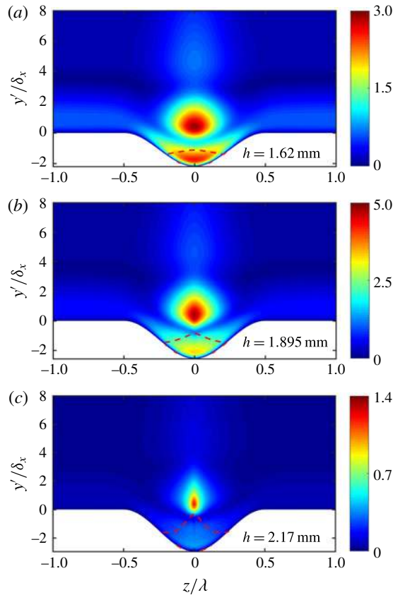
FIGURE 13. (Colour online) Comparison of |\tilde{u}'(x'_c, y', z')|/A'(x'_{neutral}, z') in the y - z planes at x' = x'_c contours where A'(x'_{neutral}, z') means amplitude of TS waves at the lower branch of the neutral stability curve. The parameter \lambda = 81 mm. (a) h = 1.620 mm; (b) h = 1.895 mm; (c) h = 2.170 mm. The red dashed lines indicate the interfaces of the regions enclosed by \Gamma = \{(y', z') : \bar{u}'(x'_c, y', z') = 0\} (zero streamwise velocity line).
