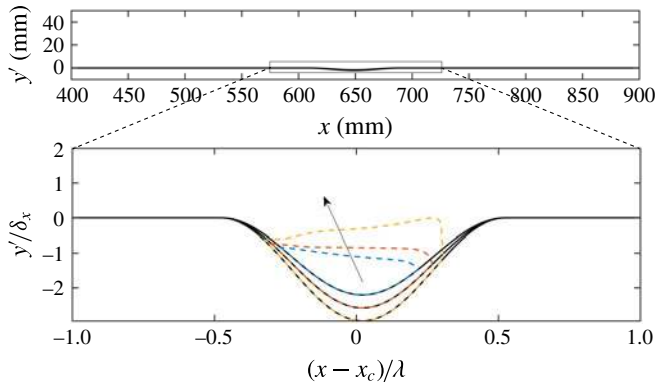
FIGURE 3. (Colour online) Relative indentation variation and associated separation bubble topological change in the plane z' = 0 for the 3-D cases with \lambda = 81 mm. For each h , the coloured dashed lines indicate the closed curves defined by \Gamma = \{(x', y') : \bar{u}'(x', y', z' = 0) = 0\} . The arrow indicates expansion of separation bubble extent with increasing h (corresponding to table 1 parameters of Group 1).
