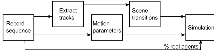
Fig. 1. Method workflow.
