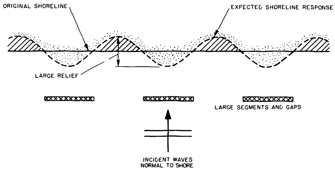
a. Large-amplitude shoreline sinuosity
