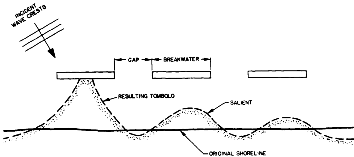
b. Segmented detached breakwater (three segments)
