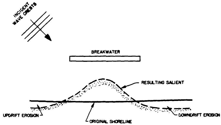
a. Single detached breakwater
