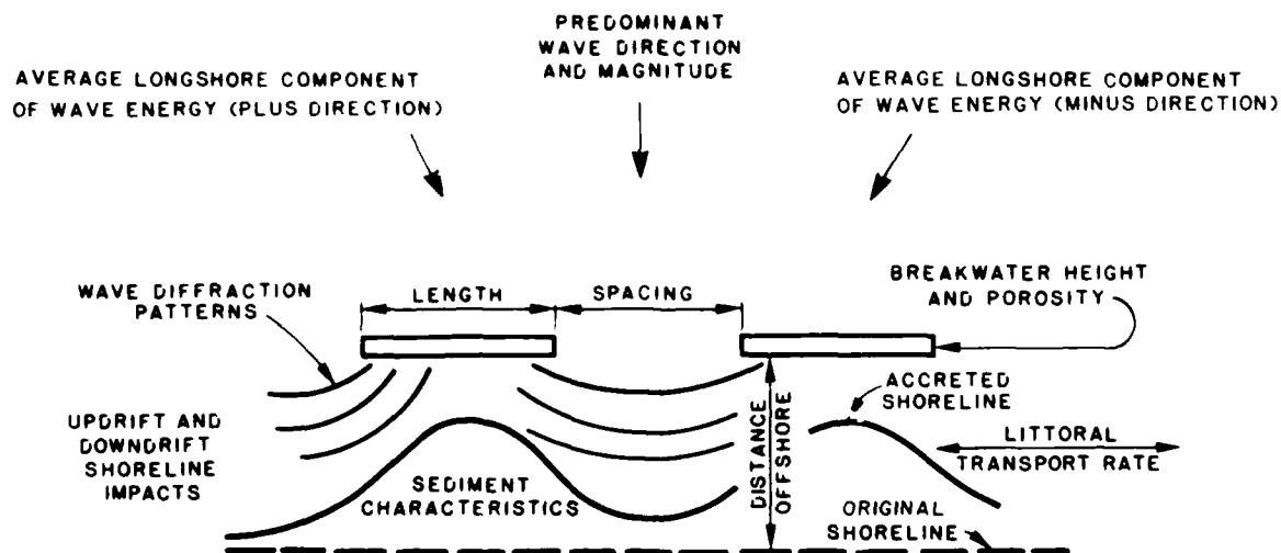
Figure 2. Segmented detached breakwater design considerations
