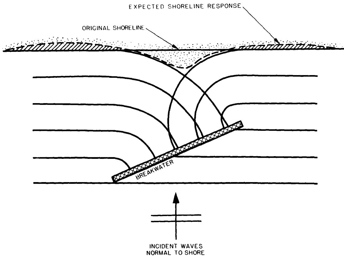
Figure 22. Effect of structure orientation on salient
