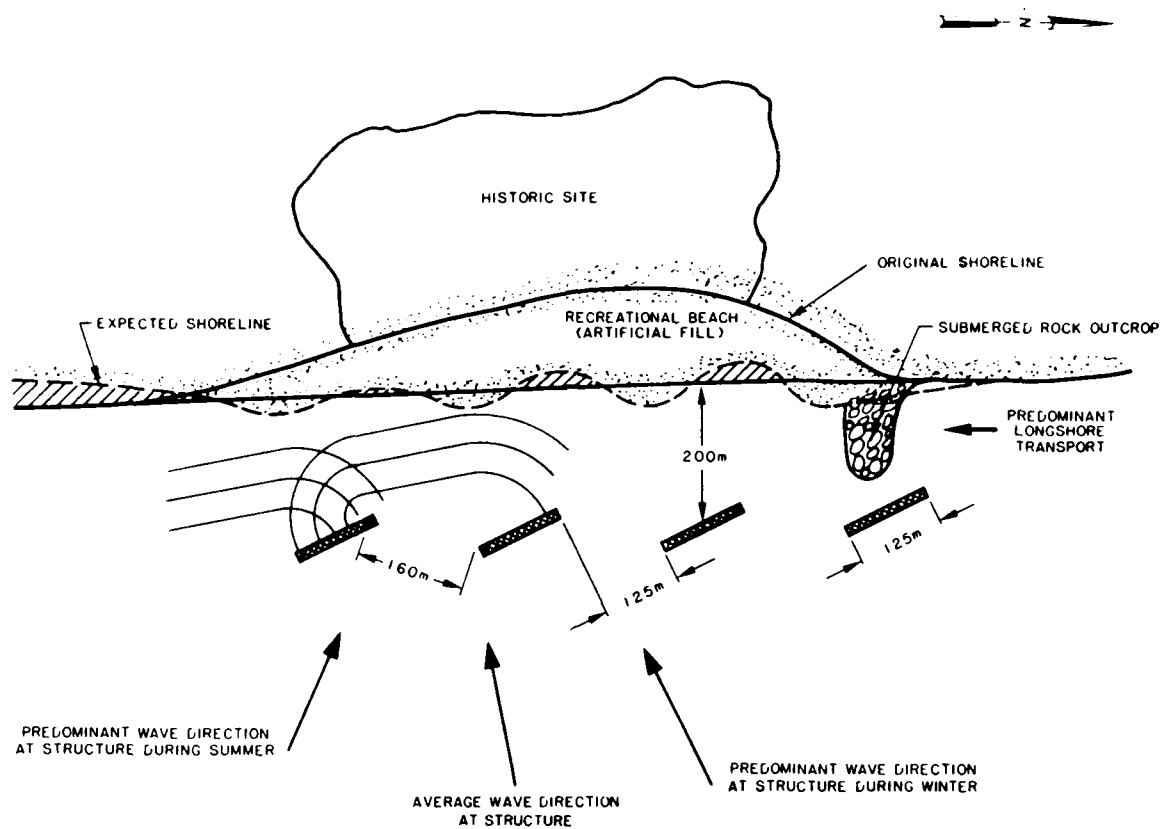
Figure B2. Layout of design for a series of unconnected salients transported through the project area to avoid such problems. A protection scheme should be devised by the use of a detached breakwater that will halt the erosion of the historic site and provide a recreational beach without any adverse effects to the adjacent nonpark property.
