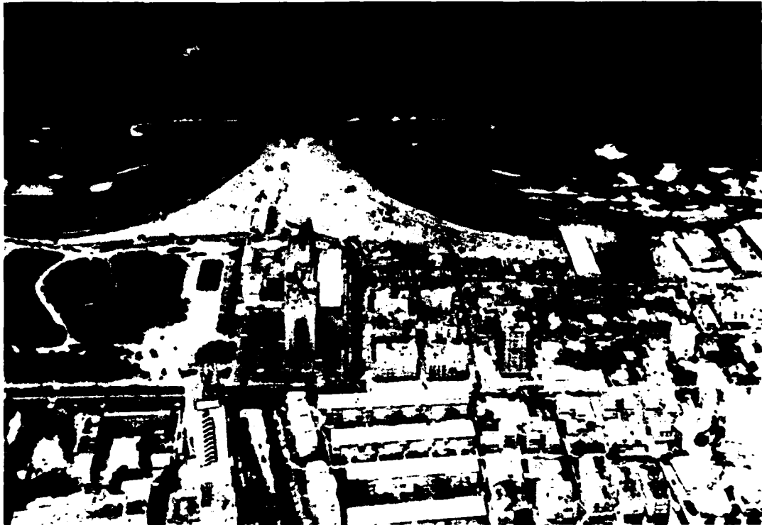
Figure 3. Breakwater and nearly symmetric tombolo (incident waves normal to shore), Tel-Aviv, Israel
