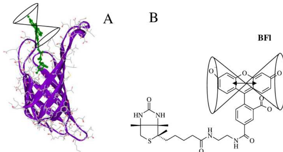
Fig 11. Pictorial representation of the AV-BFL complex. (A) The fluorescein dye in the complex has a relative high dye mobility with a half apical angle [88] ( \Omega ) of 51^\circ \pm 2^\circ in contrast with the unrestricted mobility ( 90^\circ ) of the dye in the unbound BFL. (B) The figure reflects rotational motion of the transition moment of the isoalloxazine ring system within the cone. The dye structure was added using Accelrys DS visualizer 2.0 to the AV-B crystal structure complex: 2AVI [32]. Figures only show one binding site for clarity purposes.
