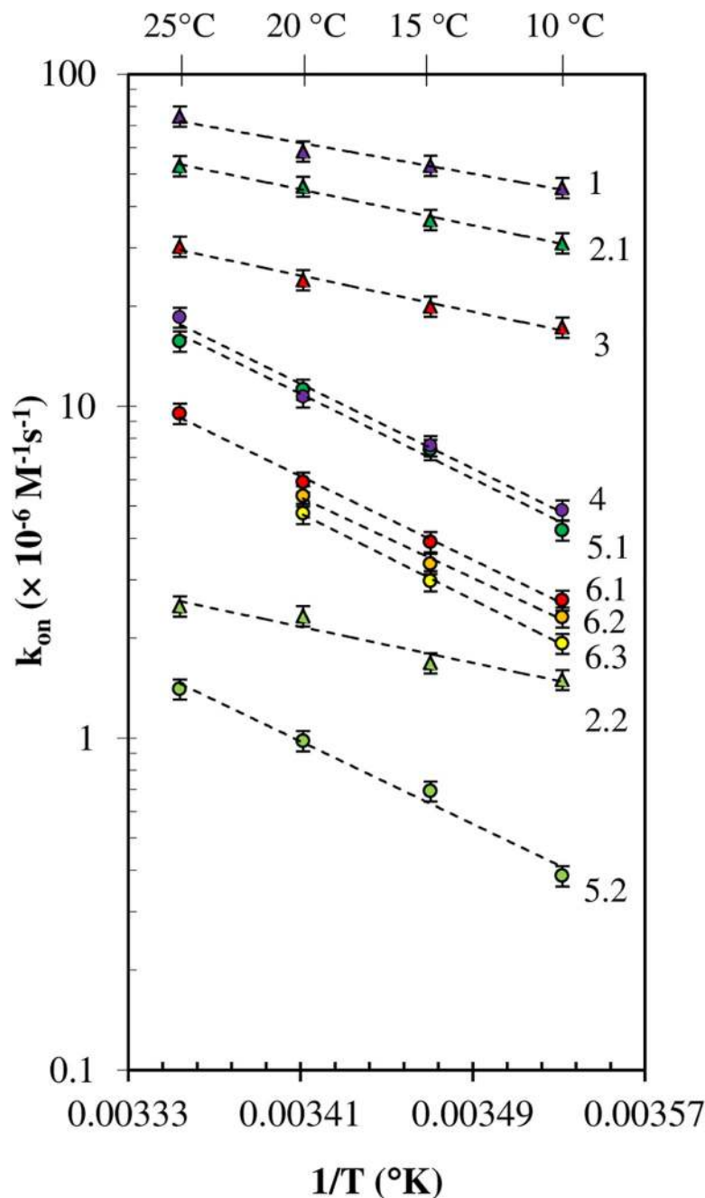
Fig 8. Arrhenius plot of the association rate constants. Temperature dependence of the B 7 association reaction at pH 8 (unless otherwise specified) for: 1 SAV-BFl (purple triangles); 2 SAV-B 7 -DNA ds *Fl (green triangles): 2.1 (k on1 ) and 2.2 (k on2 ); 3 SAV-BcO (red triangles); 4 AV-BFl (purple circles); 5 AV-B 7 -DNA ds *Fl (green circles): 5.1 (k on1 ) and 5.2 (k on2 ); 6 AV-BcO (red circles): 6.1 at pH 8, 6.2 at pH 9 (orange circles), 6.3 at pH 10 (yellow circles). The data points were plotted in semi-logarithm (ln k on vs 1/T) for clarity.
