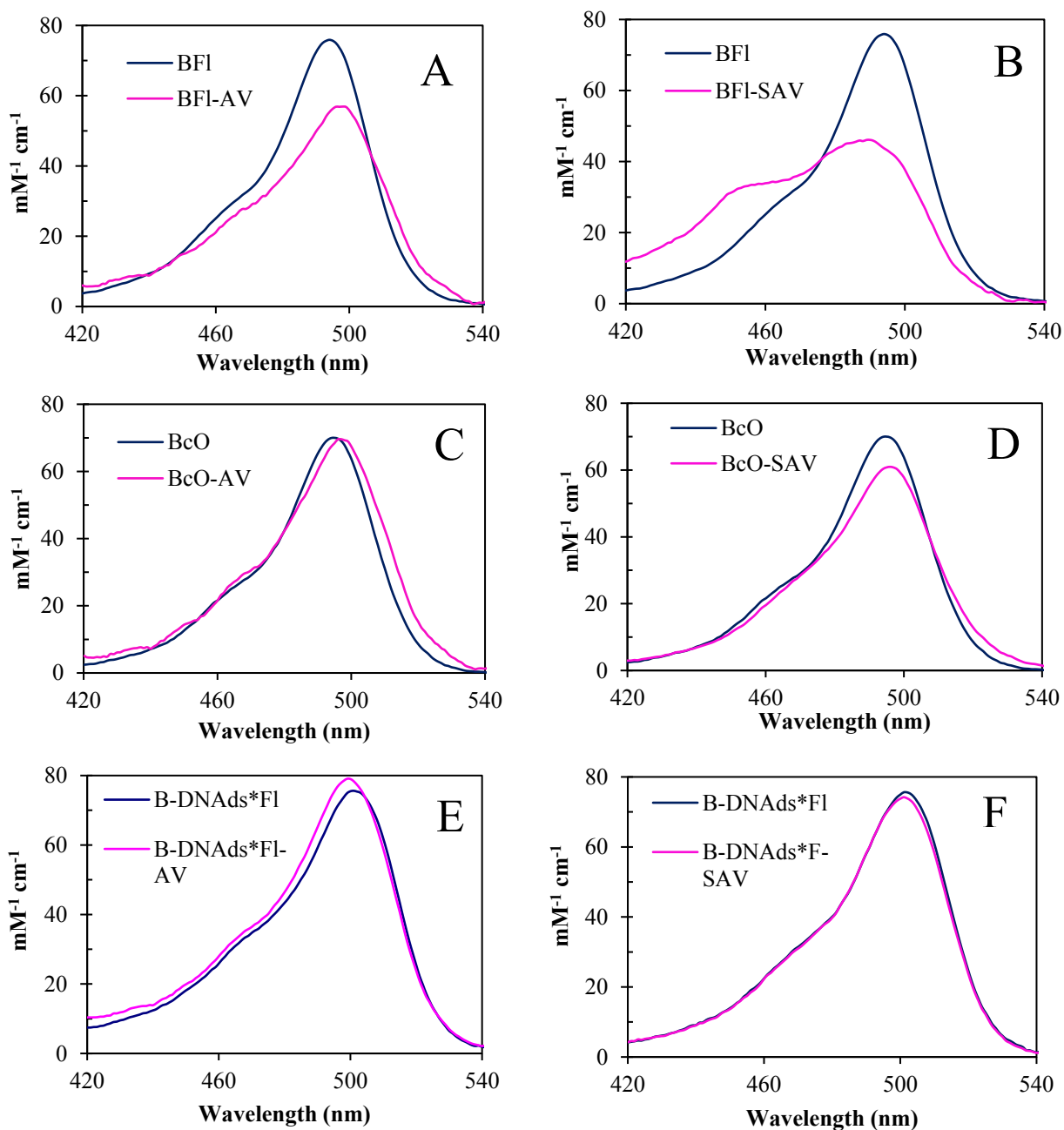
S1 Fig. Absorbance spectra of dye-labeled B 7 probes and respective complexes with AV and SAV. The absorbance spectra of the unbound BFI, BcO and B 7 -DNA ds *FI are shown in dark blue and the respective bound complexes formed with SAV and AV in pink. The spectra are normalized to the calculated molar absorptivities. The distortion of the SAV-BFI absorbance spectrum (B panel) is caused by the presence of FI 2- and FI 1- . The labeled probes and protein concentrations were 1 μM and 10 μM, respectively.
