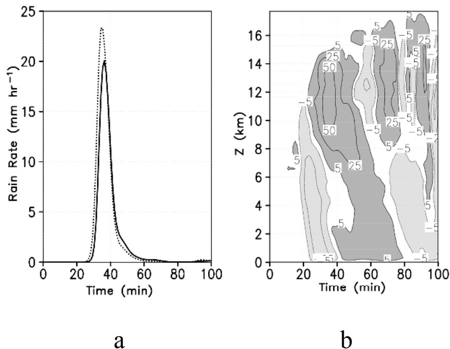
Fig. 10. (a) Surface precipitation rate (mm/hour) in the domain (grid 100–200). Dot is for Case F and solid for Case D, respectively. (b) Percentage changes (percent) in rain rate vertical profile in the domain (grid 100–200). Contours are at -50, -25, -5, 5, 25, and 50%. Light shaded area: <-5%; darker shaded area: >5%.
