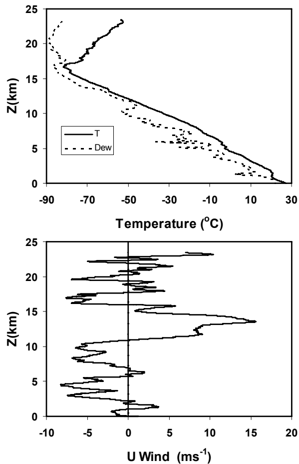
Fig. 1. Initial vertical profiles of (a) temperature (solid; ^{\circ}\text{C} ) and dew point (dashed); and (b) u wind ( \text{m/s} ) observed at -23^{\circ}\text{W} and 9^{\circ}\text{N} on 19:31 UTC 01, July 2006.
