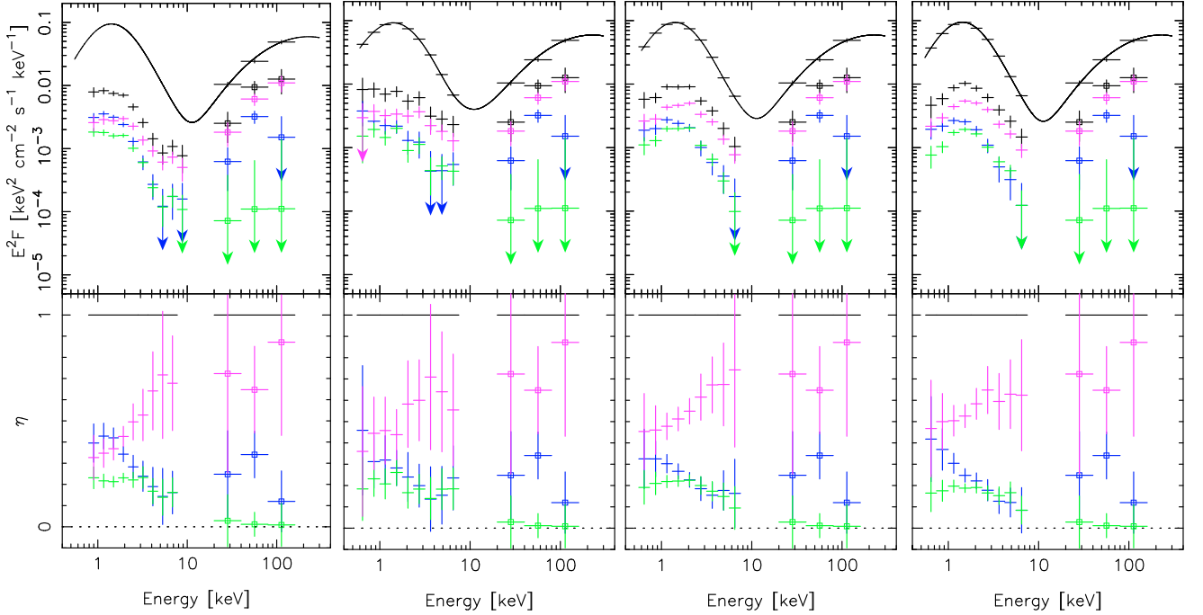
Fig. 9. For four (soft) X-ray and INTEGRAL observations shown are the total, total-pulsed and phase-resolved pulsed spectra ( top panels ) and \eta ( bottom panels , defined as the fraction of the total pulsed emission). The (soft) X-ray data from left to right are ASCA GIS, XMM-Newton PN obs. A, B and C. All data are equally binned for comparison. For the total spectra, the best fit is shown. In the top panel for ASCA-GIS the best fit to the XMM-Newton-B-INTEGRAL total spectrum is shown for clarity. The total spectra and total-pulsed spectra are plotted in black. The phase resolved spectra for Ph I, Ph II and Ph III (see Table 6) are plotted in blue, green and magenta, respectively. The INTEGRAL phase-resolved spectra are indicated in each figure with a square symbol. The data points with arrows indicate that the flux values have significances less than 1.5\sigma . The positive 1\sigma error is drawn. In the bottom panels \eta is presented in the same colour scheme as the spectra.
