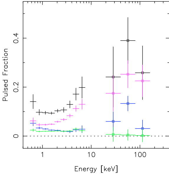
Fig. 10. Pulsed fraction as function of energy. Below 10 keV the averaged XMM-Newton pulsed fraction of observations A, B and C are plotted. Above 10 keV the INTEGRAL pulsed fraction is plotted. Colour coding as in Figs. 8 and 9; Total-pulsed emission (black), Ph I (blue), Ph II (green), Ph III (magenta).
