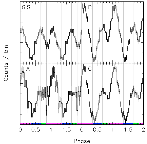
Fig. 6. 4U 0142+61 pulse profiles for 2.0–8.0 keV of ASCA-GIS and the three XMM-Newton observations (A, B, C, Table 3). The relative normalization scales approximately with the total pulsed flux (2–8 keV; see e.g. Table 8). See also the caption of Fig. 5.
