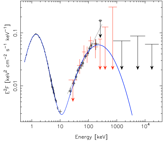
Fig. 3. Unabsorbed total spectra of 4U 0142+61 as measured with different instruments; XMM-Newton (Obs B; 0.55–11.5 keV) in black; INTEGRAL-ISGRI (Revs. 142–468; 20–300 keV) in black with open square symbols; INTEGRAL-SPI (20–1000 keV) in red; and CGRO COMPTEL (0.75–30 MeV) limits in black. Shown are also the best single power-law model fit for the ISGRI data-points (in grey) and the “three logparabola” fit for the whole band (in blue). See Sect. 3.1 for details.
