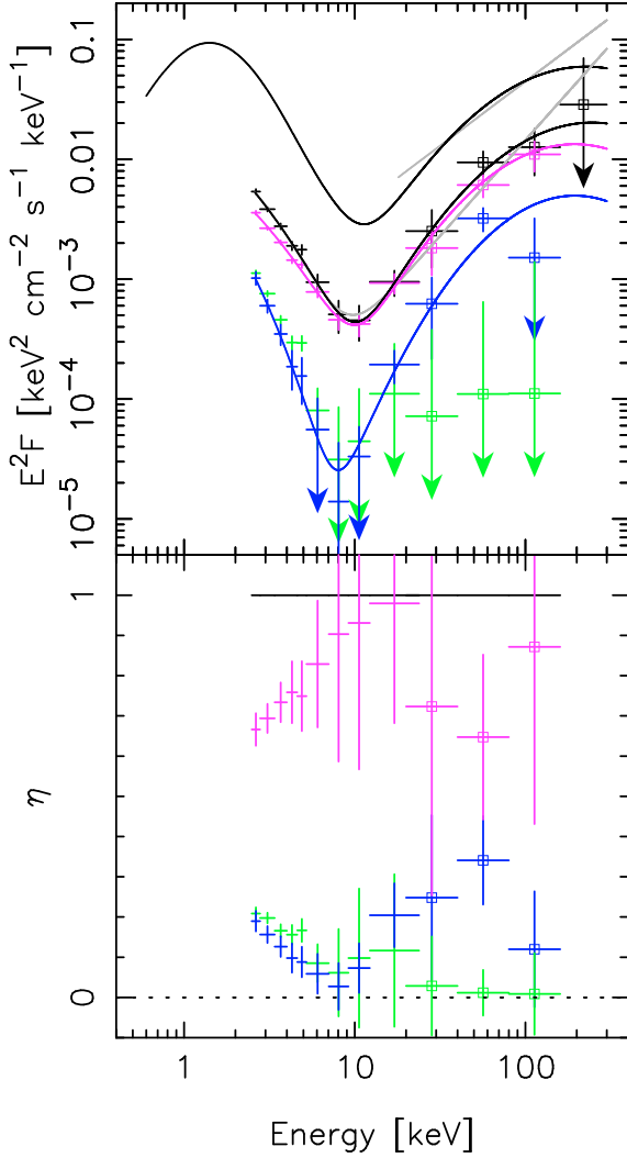
Fig. 8. In the top panel the phase-resolved pulsed-emission spectra and fits of INTEGRAL and RXTE-PCA are presented. Data points with square symbols are INTEGRAL measurements and those without a marker are from RXTE-PCA. Black is the total-pulsed spectrum; in blue Ph I; in green Ph II; and in magenta Ph III. The arrows indicate the flux measurements with a significance less than 1.5\sigma . For comparison the INTEGRAL/XMM-Newton-B total-spectrum fit is shown in black. In grey is plotted the power-law fit for the INTEGRAL total-spectrum and the power-law fit for the total-pulsed spectrum. In the bottom panel \eta is presented in the same colour scheme as the spectra. \eta is defined as the fraction of the pulsed emission in a selected phase interval Ph I, Ph II or Ph III of the total-pulsed emission, i.e. the sum equals unity.
