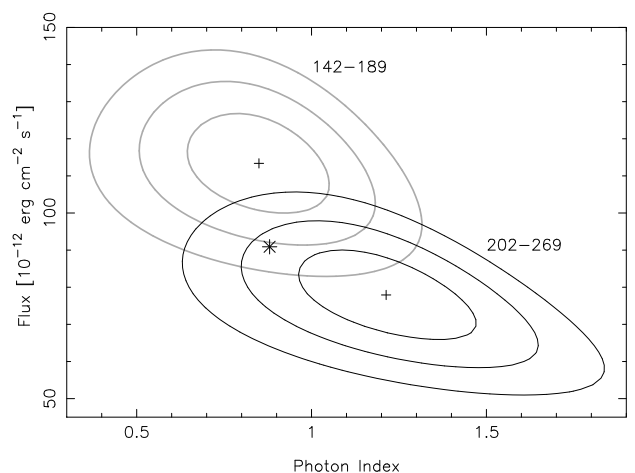
Fig. 2. Error contours ( 1\sigma , 2\sigma and 3\sigma ) of observations 142–189 (in grey) and 202–269 (in black) with respect to the time-averaged measurement (star).
