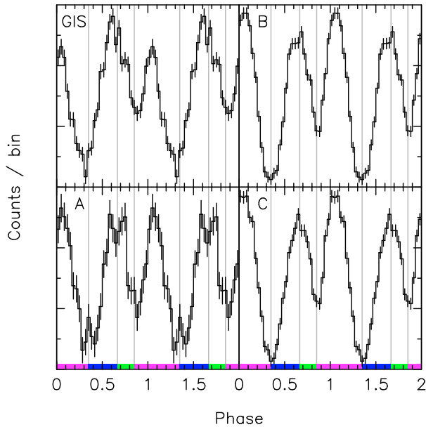
Fig. 5. 4U 0142+61 pulse profiles for 0.8–2.0 keV of ASCA-GIS and the three XMM-Newton observations (A, B, C, Table 3). Phase intervals indicated as in Fig. 4. The profile of XMM-Newton observation C required a shift in phase by -0.028 for alignment with the profile of observation B (consistent with the other profiles). The relative normalization is consistent with the total pulsed flux (0.8–2.0 keV) being approximately constant (see Table 8).
