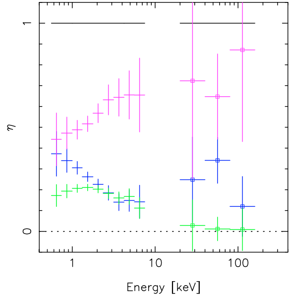
Fig. 11. Contribution to the total-pulsed emission \eta of the three selected phase intervals from the averaged XMM-Newton \eta of observations A, B and C and for INTEGRAL (>10 keV). Colour coding as in Fig. 10.
