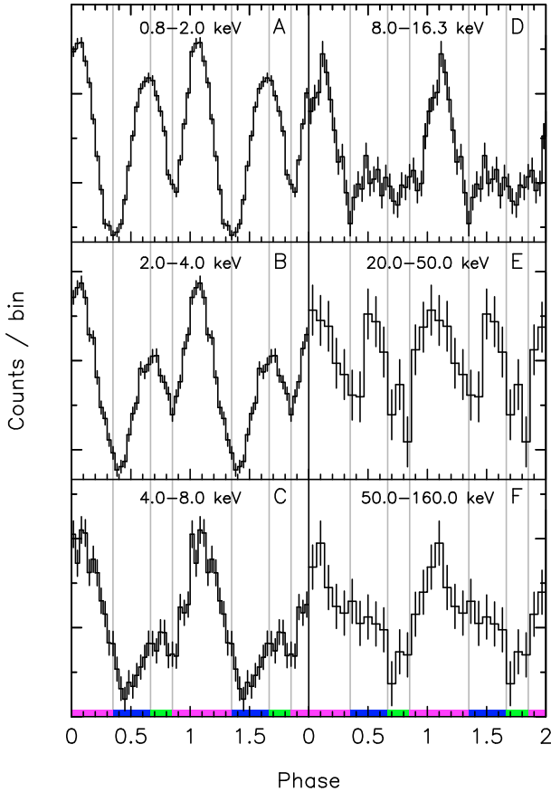
Fig. 7. 4U 0142+61 pulse profiles from soft to hard X-rays. In panels A, B and C, pulse profiles in the energy ranges 0.8–2.0 keV, 2.0–4.0 keV and 4.0–8.0 keV are shown which are the sums of the XMM-Newton observations A, B, and C. Panel D presents the RXTE-PCA pulse profile in the energy band 8.0–16.3 keV taken from Kuiper et al. (2006). In panels E and F INTEGRAL pulse profiles are shown in the energy ranges 20–50 keV and 50–160 keV. Phase intervals are indicated as in Fig. 4.
