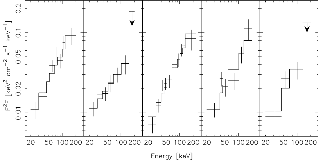
Fig. 1. Total-flux spectra of 4U0142+61 taken during INTEGRAL revolutions ( from left to right ): 142–189, 202–269, 331–336, 384–396 and 452–468. Data points are binned to 4\sigma if the single bins are of less significance. The upper limits represent 2\sigma confidence levels.
