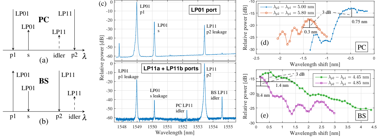
Fig. 2. (a) and (b) wavelength configurations of PC and BS, respectively; the arrows indicate gaining (up) and losing (down) power; (c) MDMUX spectra for \lambda_{p2} = 1553.45 nm and \lambda_s = 1550.15 nm; (d) and (e) idler power relative to signal power vs. idler wavelength shift for PC and BS, respectively.
