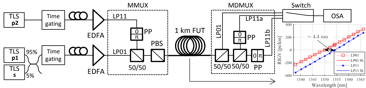
Fig. 1. Experimental setup. 50/50 denotes a non-polarization beam splitter. The inset shows measured relative inverse group velocities (RIGVs) of the LP01 and LP11 mode-groups.
