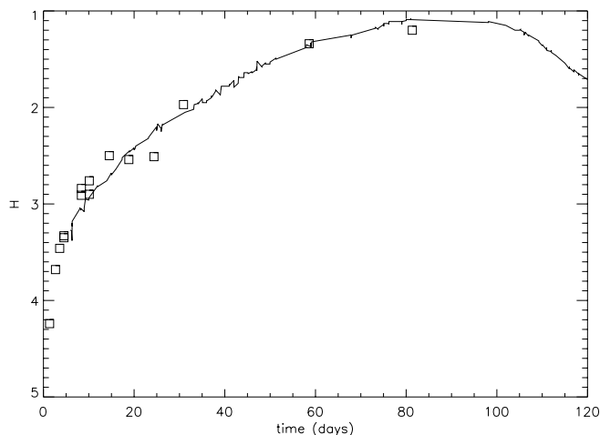
FIG. 26.—Same as Fig. 25 but for the observed H light curve
