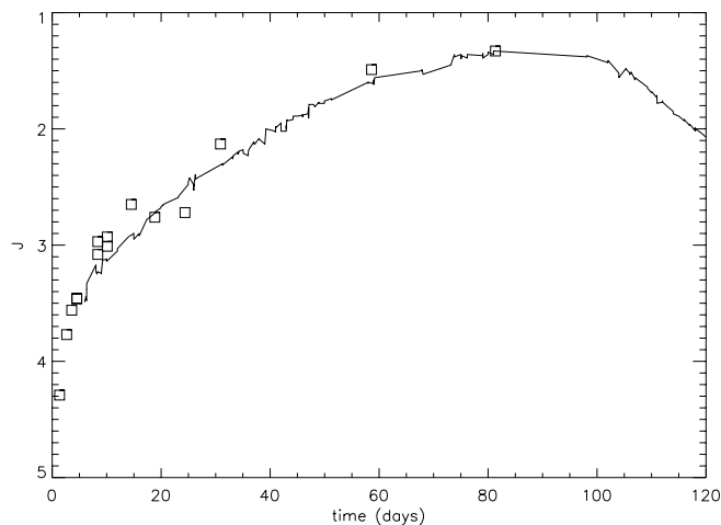
FIG. 25.—Observed J light curve of SN 1987A (solid line; Bouchet et al. 1989) is compared with the model values (squares).
