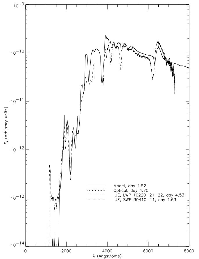
FIG. 4.—PHOENIX model spectrum for day 4.52, without additional nickel mixing.
