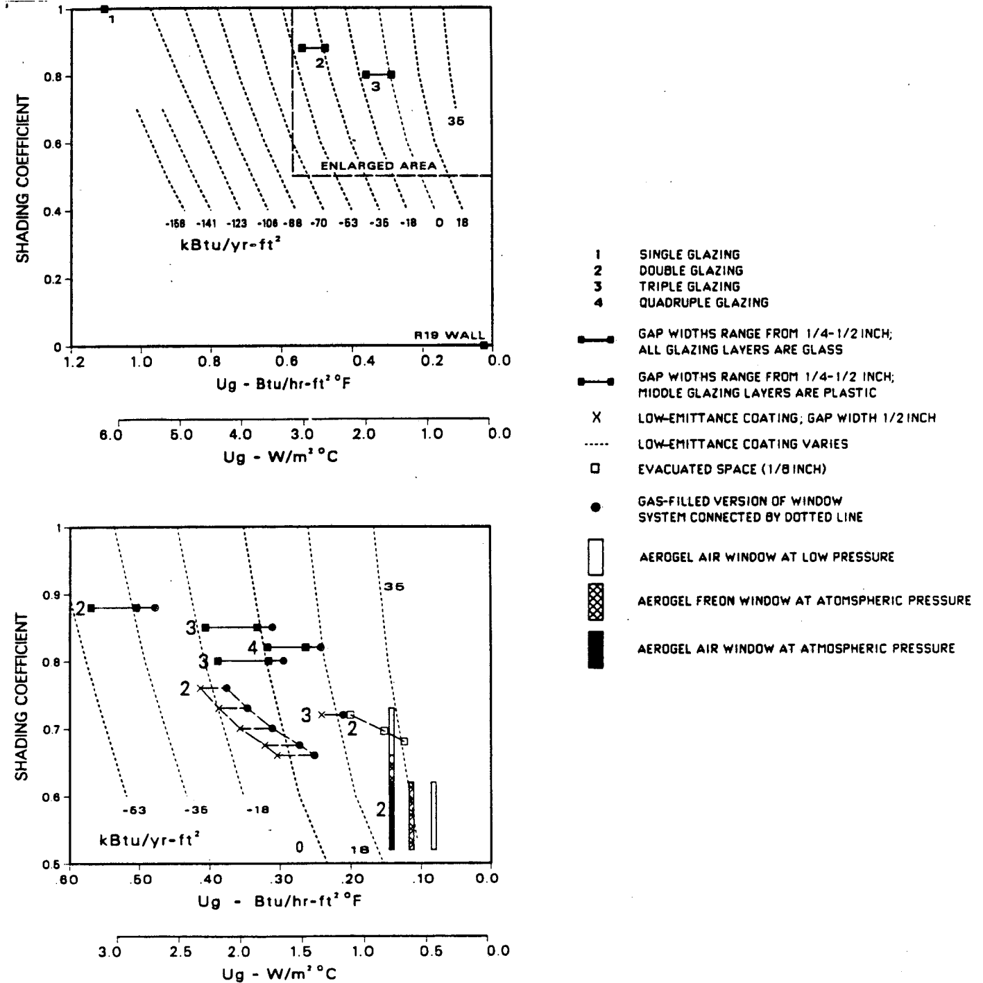
Figure 9: Net annual useful energy flux in \text{kBtu}/\text{yr}\cdot\text{ft}^2 of window area ( 1 \text{ kBtu}/\text{yr}\cdot\text{ft}^2 = 11.4 \text{ MJ}/\text{yr}\cdot\text{m}^2 ) through 66 \text{ ft}^2 ( 6.1 \text{ m}^2 ) of east-facing double- and triple-glazed and highly insulating window systems in a prototypical house in Madison, WI, expressed as a function of window U-value.
