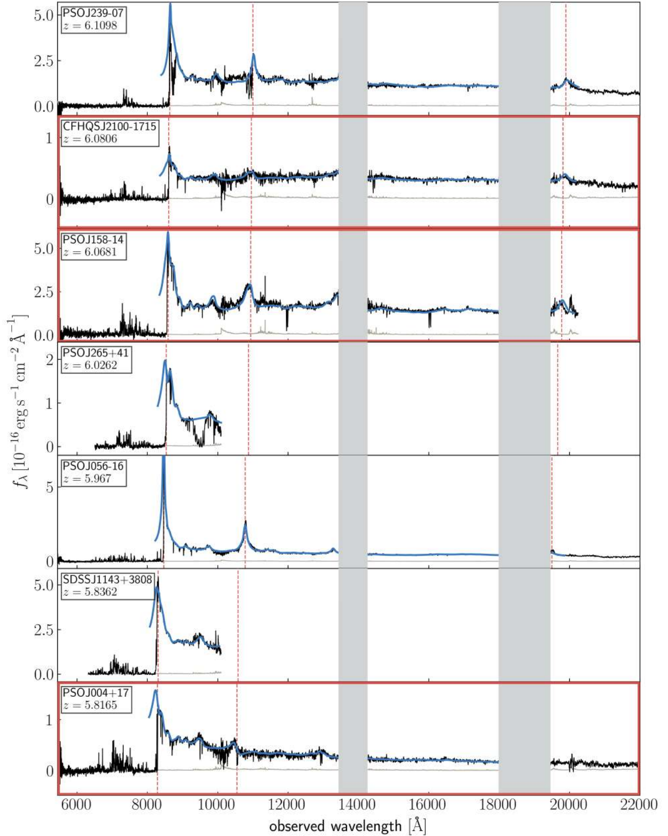
Figure 11. Same as Fig. 3 with quasar continuum estimates, shown in blue.
