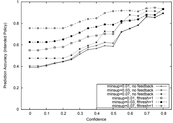
Figure 2: Prediction accuracy (intended policy)
