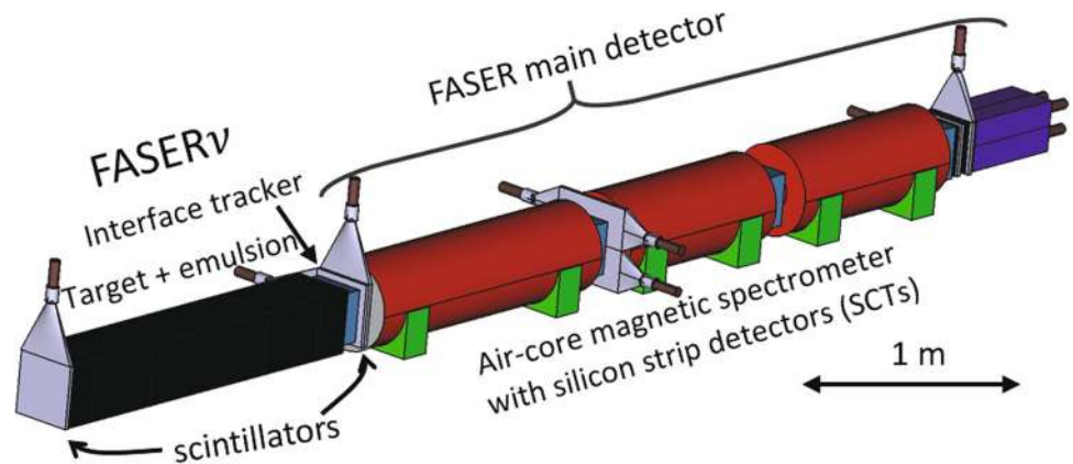
Fig. 12 Plan of the detector upgrade to couple \text{FASER}\nu to the \text{FASER} main detector. The components include the \text{FASER}\nu emulsion detector (black), scintillators (gray), tracking layers (blue), magnets (red), and electromagnetic calorimeter (purple)
