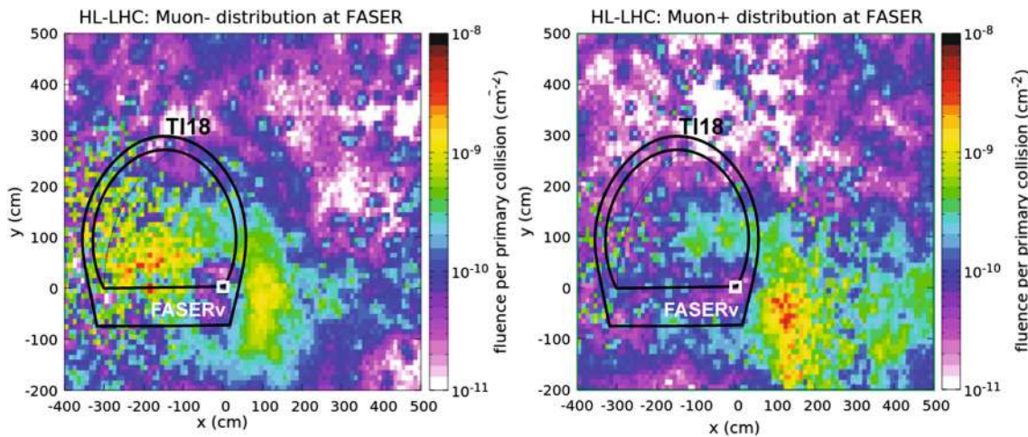
Fig. 14 Distributions of negative (left) and positive (right) muons crossing the tunnel TI18, which is in a symmetric position on the opposite side of the ATLAS IP with respect to FASERν. The position of
