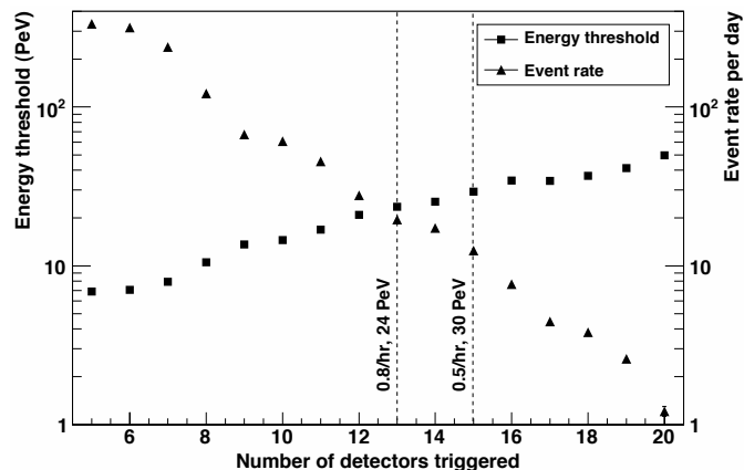
Fig. 4. Energy threshold in PeV ( left ) and the event rate per day ( right ) are shown as a function of the number of triggered particle detectors. Two possible trigger conditions are indicated with the dotted lines.
