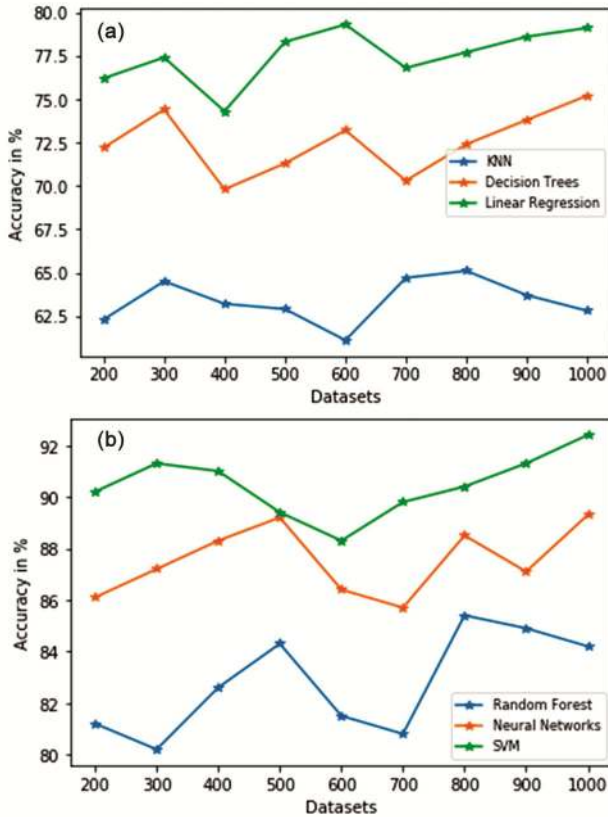
Fig. 5 — Comparison of machine learning methods: (a) KNN, Decision Tree, Linear Regression; (b) Random Forest, Neural Networks, SVM
