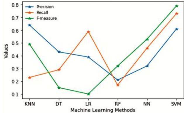
Fig. 6 — Comparison of Precision, Recall and F-measure for all machine learning methods
