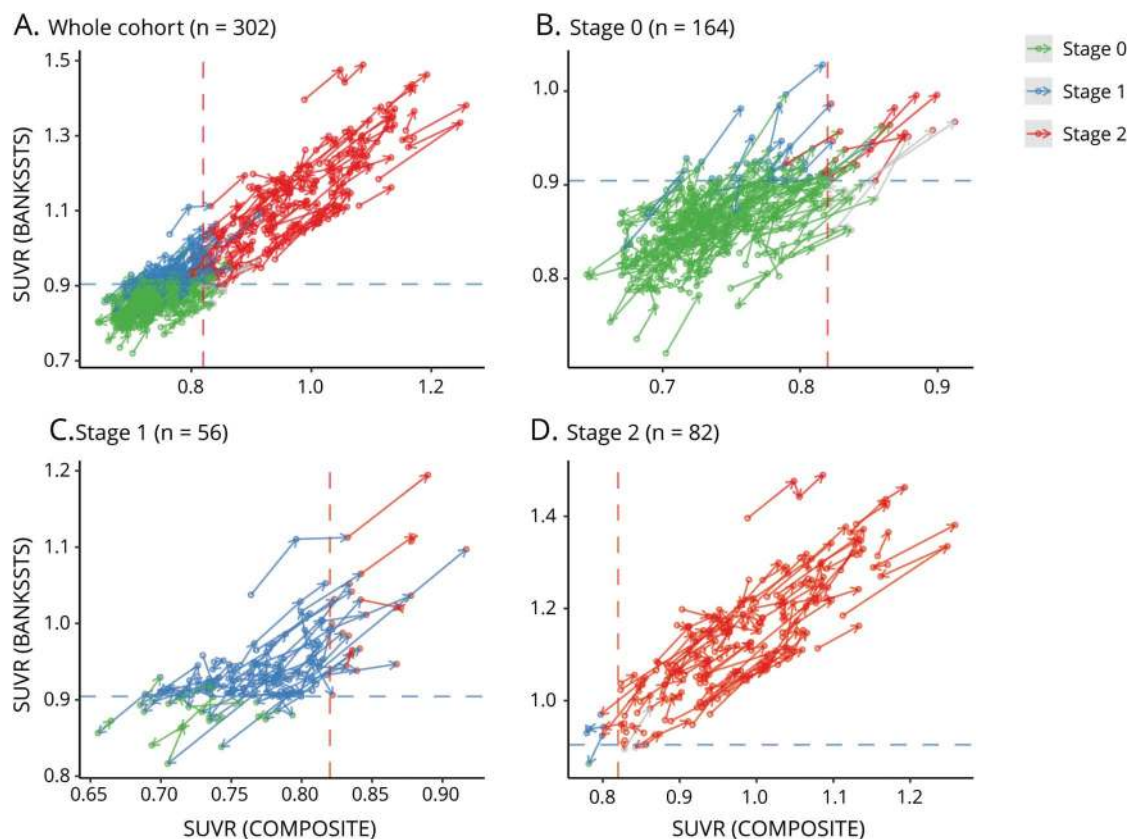
Figure 4 Transition of amyloidosis stages from different initial stage
