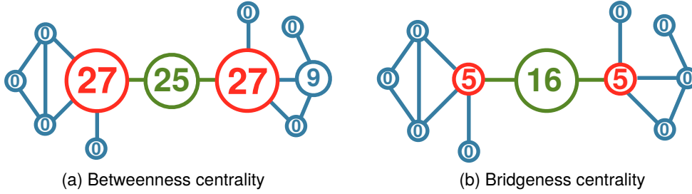
FIG. 1. The figures show the betweenness (a) and bridgeness (b) scores for a simple graph. Betweenness does not distinguish centers from bridges, as it attributes a slightly higher score (Figure a, scores = 27) to high-degree nodes, which are local centers, than to the global bridge (Figure a, score = 25). In contrast, bridgeness rightly spots out the node (Figure b, score = 16) that plays the role of a global bridge.
