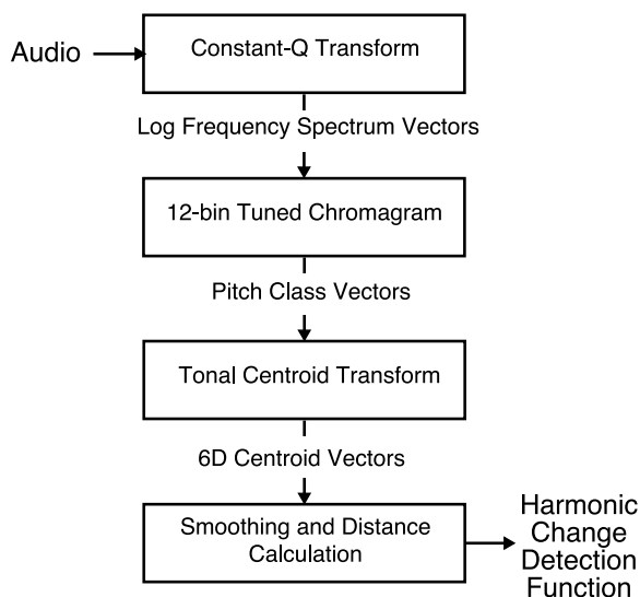
Figure 1: Flow Diagram of HCDF System.
