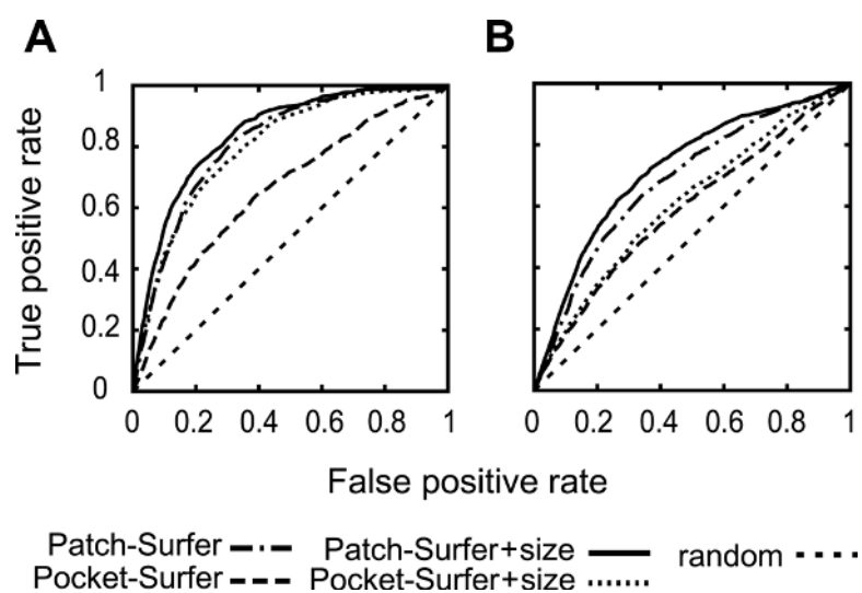
Figure 4. ROC curves of Pocket-Surfer and Patch-Surfer using the shape and the size information. A , the Kharaman dataset. B , the Huang dataset. The AUC values of the curves are shown in Table 2. The patch radius was set to 5\text{\AA} . A random retrieval yields the AUC of 0.5.
