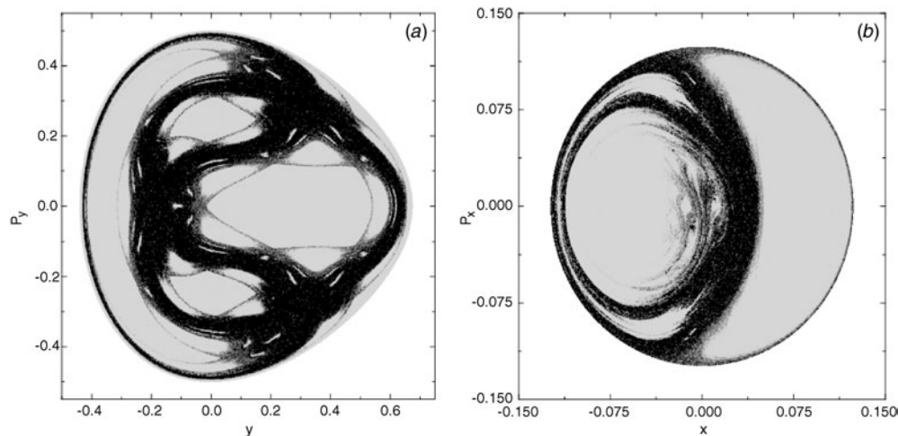
Figure 9. Regions of different values of the SALI (a) on the PSS x = 0 of the 2D Hénon–Heiles system (3), at t = 1000 and (b) on the subspace y = 0, p_y = 0 of the PSS z = 0 of the 3D system (5), at t = 5000 . In both frames initial conditions are coloured black if their SALI \leq 10^{-12} , deep grey if 10^{-12} < \text{SALI} \leq 10^{-8} , grey if 10^{-8} < \text{SALI} \leq 10^{-4} and light grey if SALI > 10^{-4} .
