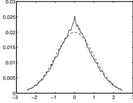
Fig. 2. Histogram of the normalized difference coefficients (solid line) and a discretized standard normal density (dashed line)
