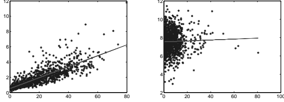
Fig. 3. Plot of \hat{Z}_x vs. \hat{Z}_d and the least-squares optimal linear fit for watermarked(left) and AWGN corrupted(right) images
