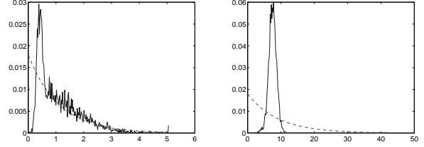
Fig. 4. Histogram of \hat{Z}_d and the best fitting discretized exponential density for watermarked(left) and AWGN(right) images
