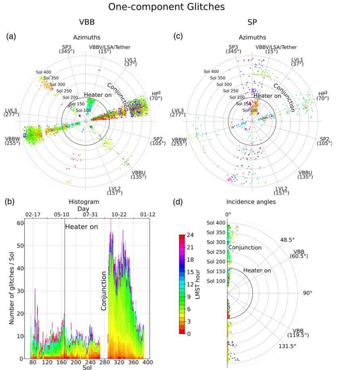
Figure 3. One-component glitches of VBB and SP for 2019 as detected by our MPS algorithm: (a) VBB one-component glitches. Glitch azimuths align with azimuths of VBB components, incidence angles are, as expected, INC \approx 48^\circ/132^\circ (not shown), (b) histogram of (a). Note the rate changes of glitches after heater activation (Sol 168) and conjunction (Sols 267–288), the latter mostly caused by VBB W, (c) SP one-component glitches for the horizontal components SP V and SP W, and (d) one-component glitches for the (almost) vertical SP U component. Color code refers to local mean solar time (LMST, in hours) of glitch onsets.
