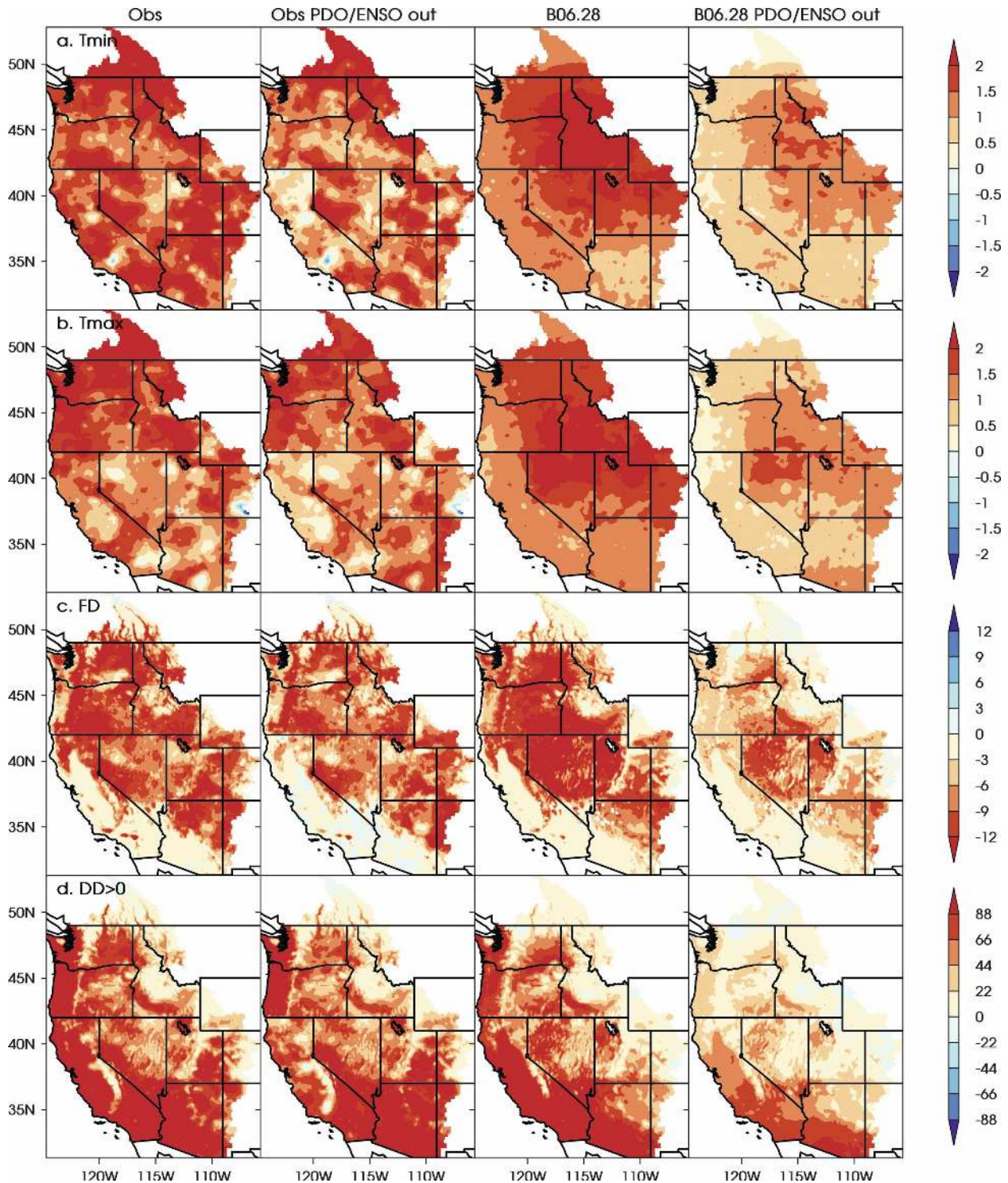
FIG. 4. Observed and one example of simulated 1950–99 changes in (a) JFM T_{\min} , (b) T_{\max} , (c) FD, and (d) DD > 0 over the western United States. Trends have been computed from the UW and one PCM-ANTH1 realization (B06.28), using raw data (columns 1 and 3) and data in which observed or simulated PDO and ENSO are regressed out (columns 2 and 4). The color scale is chosen such that red indicates an increase in T_{\min} and T_{\max} , an increase of DD > 0 , and a decrease in FD.
