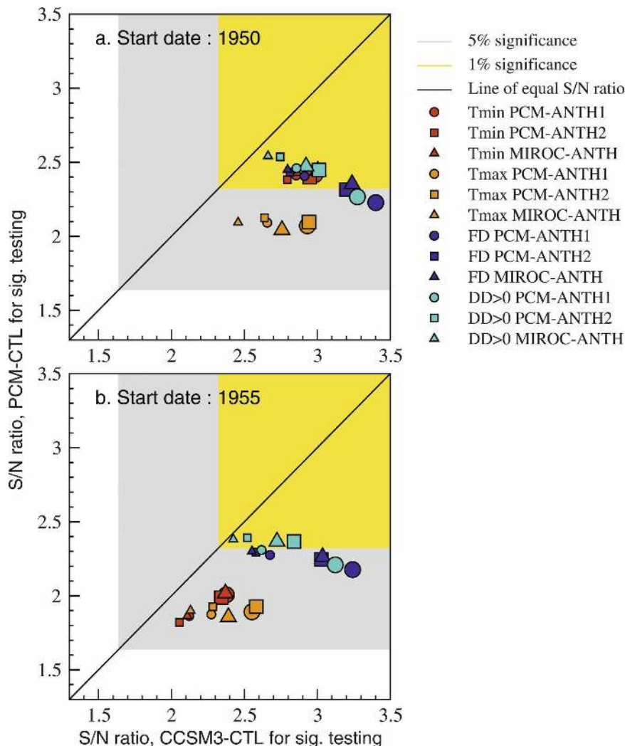
FIG. 10. Sensitivity of S/N_{50} to the variable (color), the choice of the model used to estimate the fingerprint (symbol), the method to downscale the fingerprint (circle versus square), the areal-weighting option (size), and the start year: (a) 1950; (b) 1955. CCSM3-CTL (PCM-CTL) is used for assessing statistical significance in x axis ( y axis).
