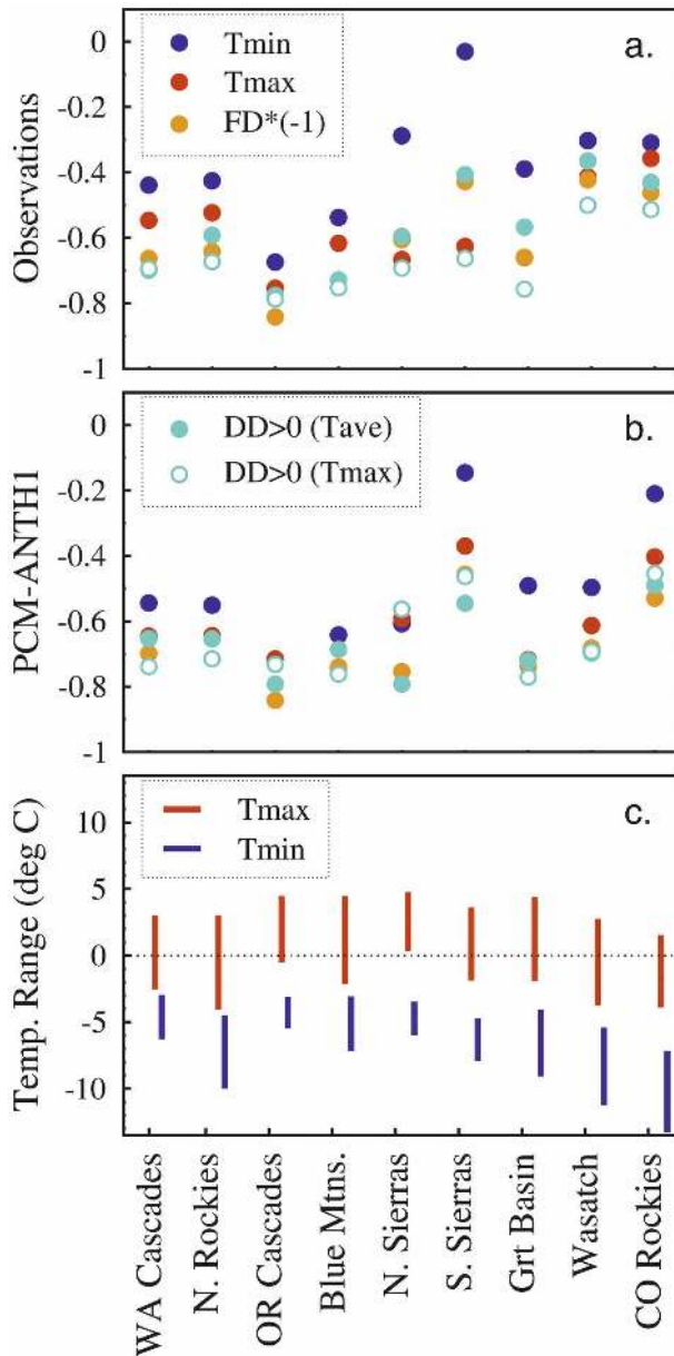
FIG. 3. Correlation between SWE/P and five different JFM temperature indices averaged over the period 1950–99 from (a) observations and (b) PCM-ANTH1 ensemble mean. (c) Range of daily observed climatological data for T_{\min} and T_{\max} computed over the period 1950–99.
