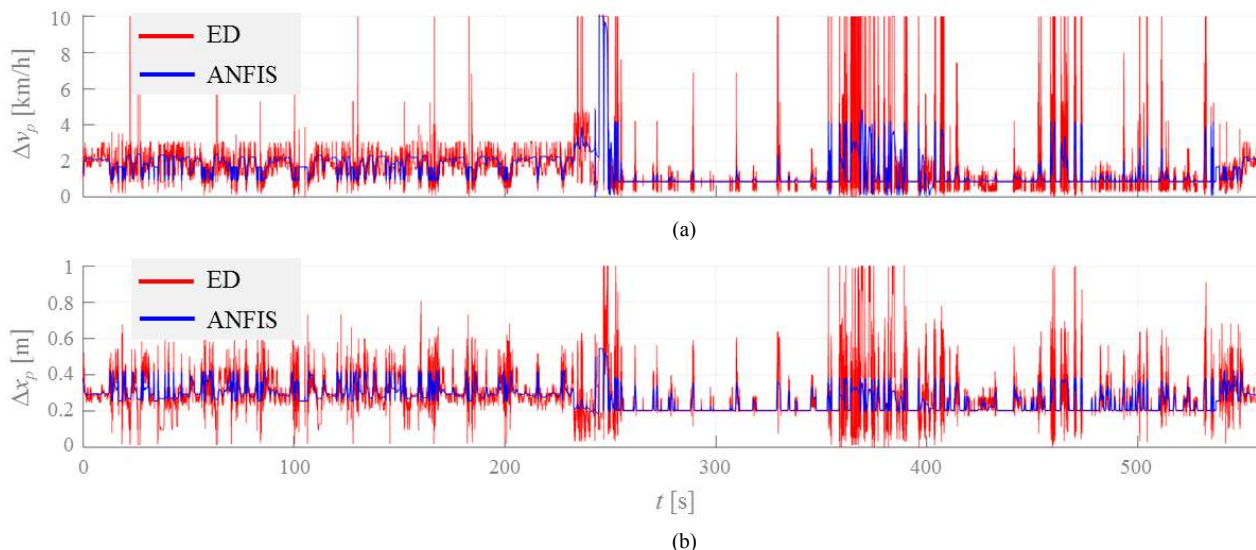
Fig 11. Driver performance prediction algorithms comparison: the red curve represents performance prediction by the ED; the blue curve displays performance prediction by the ANFIS: (a) \Delta v_p ; (b) \Delta x_p .
