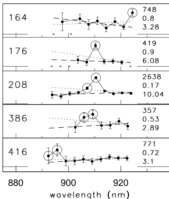
Figure 11. Top. Strip-mosaic scans showing candidate examples from a deep galaxy survey field, scanned with the TAURUS Tunable Filter (25Å passband) in conjunction with a 909/40 nm blocking filter. Circles denote aperture size and the numbers are object labels. Bottom. Narrowband fluxes for the same candidates. Numbers ( right ) are flux (in ADU), star-galaxy parameter and emission deviation (in \sigma ). Also shown are the initial ( dotted ) and final ( dashed line ) linear fit to the continuum flux. Deviant points rejected from the final fit are indicated ( circles ), as are non-detections in a frame ( crosses ). The catalogue numbers ( left ) correspond to those in panel (a).
