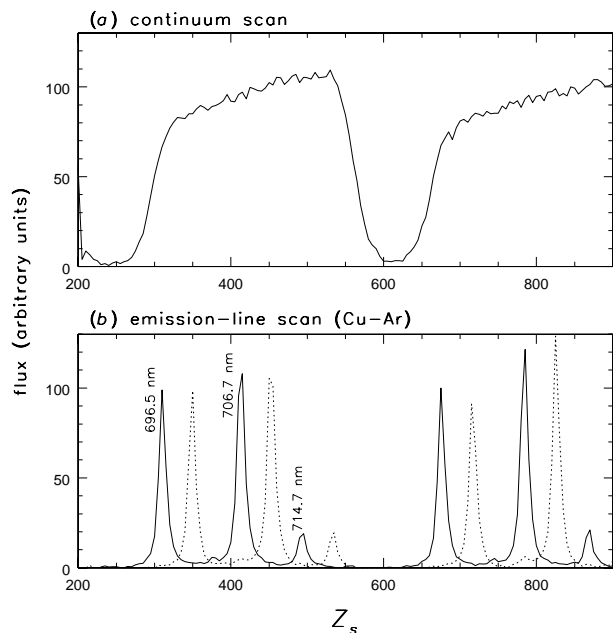
Figure 9. Example tunable filter calibration scans through the same blocking filter, showing (a) continuum, and (b) emission-line spectra. The two scans in (b) were measured on-axis ( solid line ) and off-axis ( dotted ).
