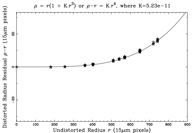
Figure 10. Radial distortion in the TAURUS-2 focal reducer of the AAT, as measured across the focal plane by C. Tinney using an MIT-LL CCD ( 15\mu\text{m} pixels). The residuals between the distorted ( \rho ) and undistorted ( r ) radii have been plotted and fit with the power law shown at top.
