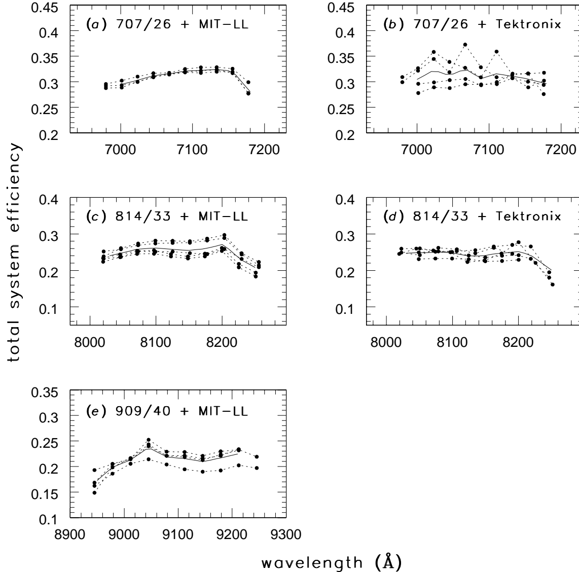
Figure 12. Measurements of total system efficiency (atmosphere + telescope + TAURUS-2) using both the MIT-LL ( a,c,e ) and Tektronix ( b,d ) CCDs. Scans through the 707/26, 814/33 and 909/40 nm blocking filters are shown. Individual scans ( dotted ) were taken on observing runs between September 1996 and April 1998. Mean values for each combination ( solid ) have also been determined. The drop in efficiency at the edges is due to the spectral cut-off of the blocking filter.
