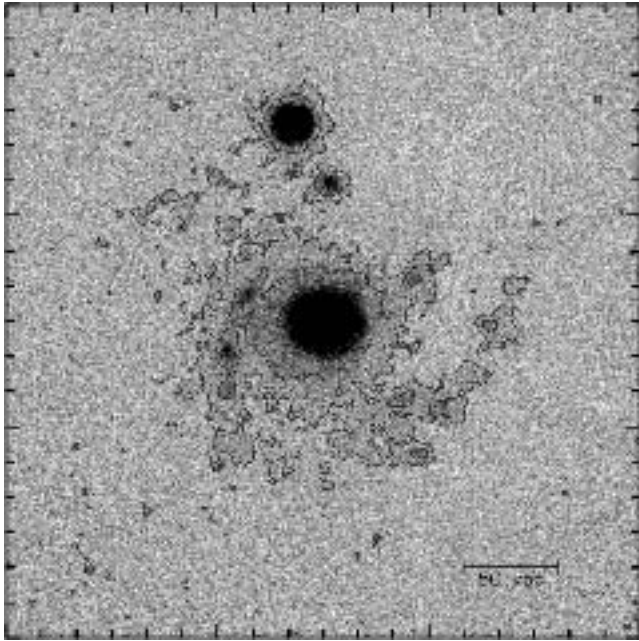
Figure 13. Deep H \alpha image showing the extended nebular emission surrounding the quasar MR2251-178. The image was obtained by Shopbell, Veilleux & Bland-Hawthorn (1999) using the Taurus Tunable Filter. The frame is 3' \times 2.5' with north up and east to the left, and reaches a flux limit of 1.8 \times 10^{-17} erg s ^{-1} cm ^{-2} arcsec ^{-2} . The faint curved structure to the south-west is real and not a residual ghost image.
