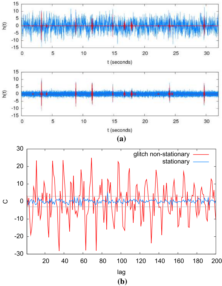
Fig. 73 Panel a shows simulated stationary AR(1) data with non-stationary noise transients, or glitches , highlighted in red . The upper panel is the raw data, while the lower panel has been whitened by the estimated amplitude spectral density. Panel b shows the autocorrelation for the stationary AR(1) data without glitches in blue , and with glitches in red
