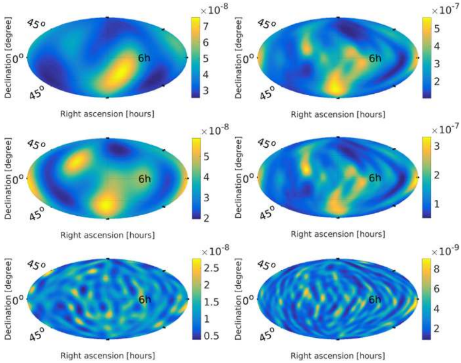
Fig. 85 90% confidence-level upper-limit maps on gravitational-wave power for anisotropic backgrounds having spectral indices \beta = 0, 2/3, and 3 (first, second, and third row, respectively). The data analyzed were from advanced LIGO’s first observational run O1 (Abbott et al. 2016a). Left column UL maps on the fractional energy density \Omega_\beta(\hat{n}) expressed in units of \text{sr}^{-1} , constructed using the spherical harmonic decomposition method out to l_{\text{max}} = 3, 4, and 16 . Right column UL maps on the energy flux F_{\beta, \hat{n}_0} expressed in units of \text{erg cm}^{-2} \text{s}^{-1} \text{Hz}^{-1} , constructed using the radiometer method, which assumes a point-source signal model. Figure adapted from Abbott et al. (2016a)
