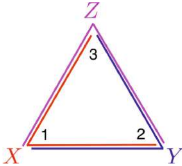
Fig. 78 Panel a shows the geometry of a LISA-like space interferometer and the laser paths for the synthetic Michelson interferometers X, Y, Z . Panel b shows sensitivity curves for the A, E, T interferometry variables compared to a scale-invariant background, \Omega_{\text{gw}}(f) = \Omega_0 = \text{const} , with \Omega_0 = 10^{-10} . The Sagnac-like T channel is far less sensitive than the Michelson-like A, E channels, and can be used to measure the instrumental noise levels. (Panel b is adapted from Adams and Cornish (2010) )
