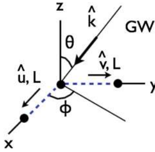
Fig. 28 Geometry for calculating the difference in the round-trip light-travel times in the two arms of a Michelson interferometer: \hat{k} = -\hat{n} is the direction of propagation for a plane gravitational wave; \hat{u} and \hat{v} are unit vectors that point from the vertex of the interferometer (e.g., the beam splitter) to the two end masses; and L denotes the lengths of each of the arms in the absence of a gravitational wave
