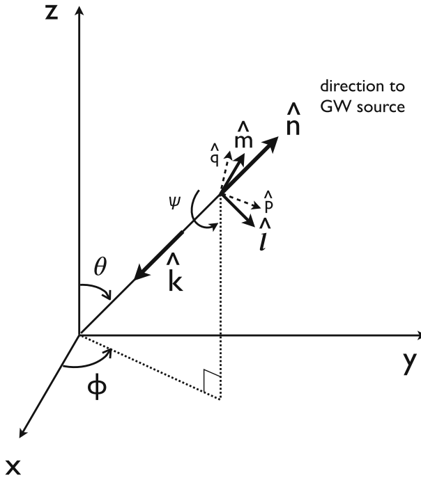
Fig. 2 Our convention for the unit vectors \{\hat{n}, \hat{l}, \hat{m}\} in terms of which the polarization basis tensors e_{ab}^+(\hat{n}) and e_{ab}^x(\hat{n}) are defined. The unit vector \hat{n} points in the direction of the gravitational-wave source (the gravitational wave propagates in direction \hat{k} = -\hat{n} ); \hat{l} = \hat{\theta} and \hat{m} = \hat{\phi} are two unit vectors that lie in the plane perpendicular to \hat{n} . Another choice for the polarization basis tensors, defined in terms of the ‘rotated’ unit vectors \hat{p} and \hat{q} , is given in Appendix A
