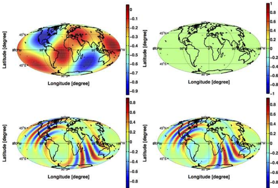
Fig. 43 Real and imaginary parts of \gamma(f, \hat{n}) (appropriately normalized) for the strain response of the 4-km LIGO Hanford and LIGO Livingston interferometers for f = 0 Hz (top two plots) and f = 200 Hz (bottom two plots). In the top left plot, note the large blue region in the vicinity of the two detectors, corresponding to the anti-alignment of the Hanford and Livingston interferometers—i.e., the arms of the two interferometers are rotated by 90^\circ with respect to one another. As shown in the top right plot, there is no imaginary component to the integrand of the overlap function at 0 Hz. The bottom two plots show multiple positive and negative oscillations (‘lobes’), which come from the exponential factor e^{-i2\pi f \hat{n} \cdot \Delta \vec{x}/c} of the product of the two response functions (5.43). The location of the positive and negative lobes are shifted relative to one another for the real and imaginary parts. The separation between the lobes depends inversely on the frequency
