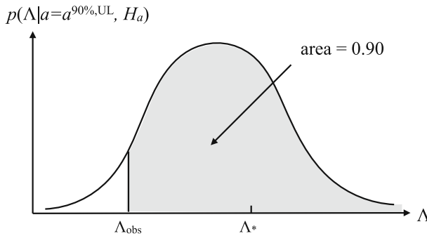
Fig. 5 Graphical representation of a frequentist 90% confidence level upper limit. When a = a^{90%,UL} , the probability of obtaining a value of the detection statistic \Lambda \geq \Lambda_{obs} is equal to 0.90
