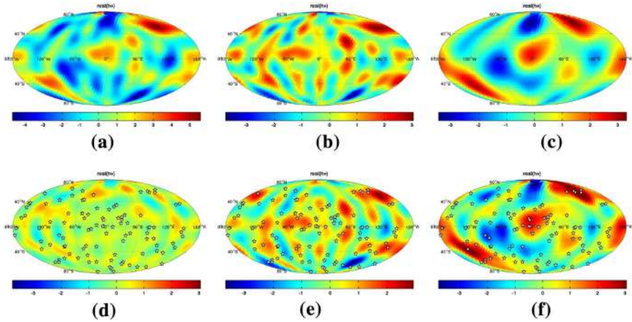
Fig. 55 Mollweide projections of the real parts of h_+(\hat{n}) for the different components of the simulated background (panels a–c ), the maximum-likelihood recovered map for a pulsar timing array consisting of N = 100 pulsars (panel e ), and the corresponding residual maps for the grad-component (panel d ) and the total simulated background (panel f ). Sky maps of the imaginary part of h_+(\hat{n}) and the real and imaginary parts of h_\times(\hat{n}) are similar, and hence are not shown in this figure. Note that the maximum-likelihood recovered map most-closely resembles the gradient component of the simulated background, since a pulsar timing array is insensitive to the curl modes of a gravitational-wave background. Image reproduced with permission from Gair et al. (2014), copyright by APS. a Total map (grad+curl). b Gradient component. c Curl component. d Gradient residual map. e Max-likelihood recovered map. f Total residual map
