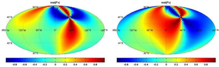
Fig. 27 Mollweide projections of the response functions R_{\text{doppler}}^+(\hat{n}) , R_{\text{doppler}}^\times(\hat{n}) , for one-way tracking Doppler frequency measurements corresponding to a pulsar located in the direction of the white star (\theta, \phi) = (50^\circ, 60^\circ) . The imaginary parts of both response functions are identically zero, so are not shown above
