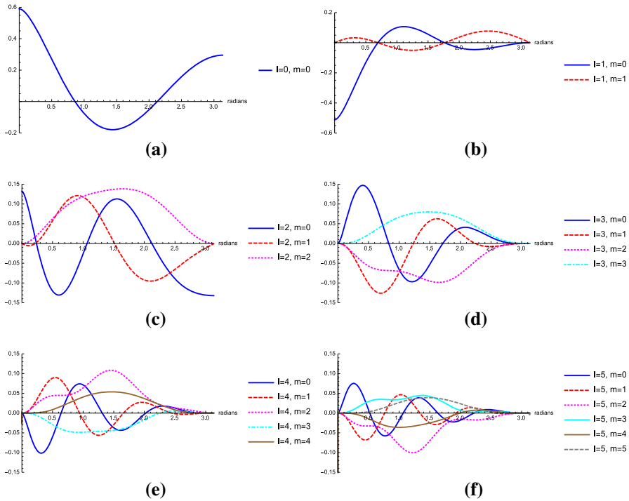
Fig. 46 Spherical harmonic component functions \gamma_{lm}(\zeta) for pulsar timing as a function of the angle \zeta between two distinct pulsars. Here we show plots for l = 0, 1, \dots, 5 and m \geq 0 . We used the Earth-term-only Doppler-frequency response (5.21) to calculate these functions
