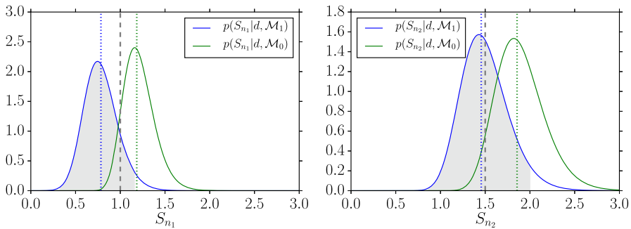
Fig. 19 Marginalized posterior distributions for the detector noise variances S_{n_1} ( left panel ) and S_{n_2} ( right panel ) for the signal-plus-noise model \mathcal{M}_1 ( blue curves ) and the noise-only model \mathcal{M}_0 ( green curves ), respectively. The actual values of S_{n_1} and S_{n_2} used for the simulation are shown by the grey dashed vertical lines . The 95% Bayesian credible intervals for the signal-plus-noise model \mathcal{M}_1 are the grey-shaded regions . For comparison, the frequentist estimators of S_{n_1} and S_{n_2} for the two models are shown by the ( blue and green ) dotted vertical lines
