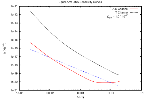
Fig. 78 Panel a shows the geometry of a LISA-like space interferometer and the laser paths for the synthetic Michelson interferometers X, Y, Z . Panel b shows sensitivity curves for the A, E, T interferometry variables compared to a scale-invariant background, \Omega_{\text{gw}}(f) = \Omega_0 = \text{const} , with \Omega_0 = 10^{-10} . The Sagnac-like T channel is far less sensitive than the Michelson-like A, E channels, and can be used to measure the instrumental noise levels. (Panel b is adapted from Adams and Cornish (2010) )
