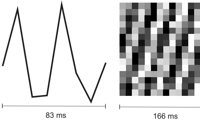
Fig. 3. Dynamic spectrum of PSR J1326+3346 ( right panel ) obtained by adding a period of 4 \times 41.5 = 166 ms for the best day using the program for the pulsar search (Tyul'bashev et al. 2016, 2017). The mean profile with the double period is presented in the left panel .
