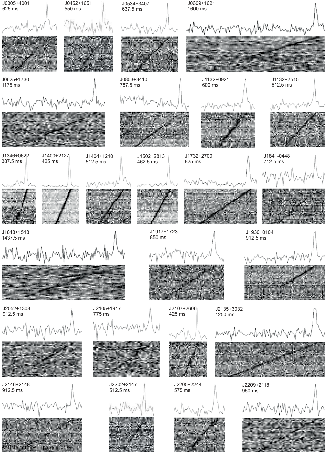
Fig. 2. 25 RRATs from Table 1. The average profile, dynamic spectrum, and recording duration are represented for each RRAT.
