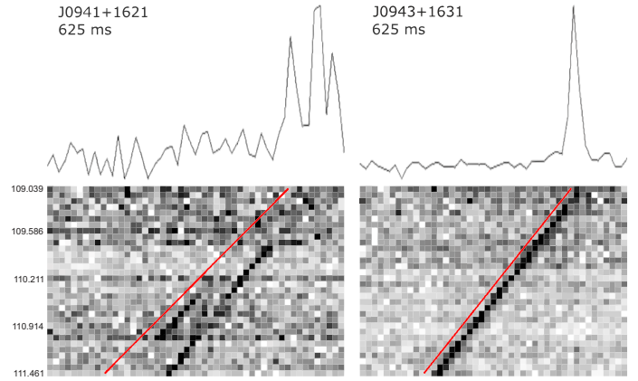
Fig. 1. Two different slopes in the dynamic spectrum in the image that corresponds to RRAT J0941+1621 and PSR J0943+1631.
