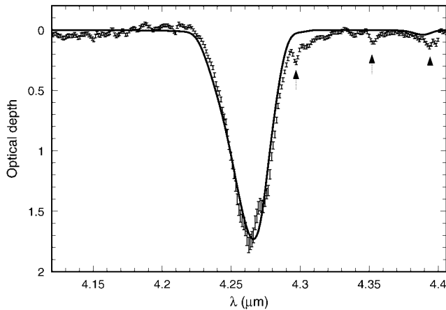
FIG. 2.—Optical depth plot (points with error bars) deduced from the SWS data in the region of the \text{CO}_2 stretching mode. Arrows indicate the positions of photospheric CO lines in the K1 III star. The solid curve is the best-fitting laboratory ice mixture ( \text{H}_2\text{O}:\text{CO}_2:\text{CO} = 100:20:3 at 20 K).
