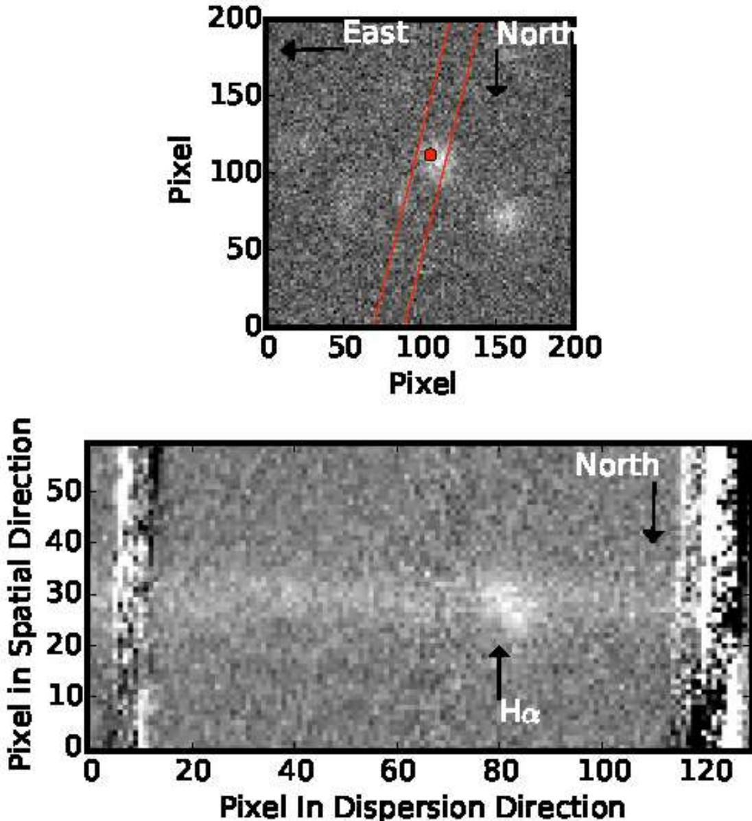
FIG. 6.— The top panel shows the DEIMOS slit (red lines) with Position Angle (PA) of 200 overlaid on iPTF13ehe (red dot) and the host galaxy. The slit width is 1.2'' . The bottom panel is the reduced 2-dimensional DEIMOS spectrum taken on December 21, 2014. The x-axis is the dispersion direction, with a scale of 0.33\text{\AA} per pixel, and the y-axis is the spatial direction with a scale of 0.1185'' per pixel.
