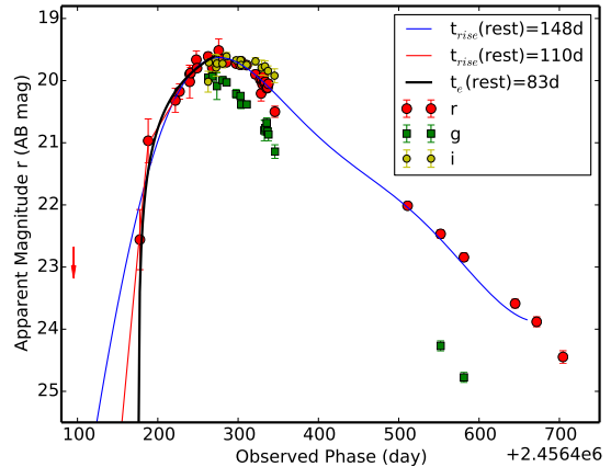
FIG. 1.— The iPTF13ehe apparent brightness in the g , r and i -band versus observed Julian date, overlaid with polynomial fits to the r -band LC in order to infer the peak and explosion dates. The blue line uses all of the data, the red line uses a piece-wise polynomial fit and the black line is based on an exponential form. The time scales are in the rest-frame.
