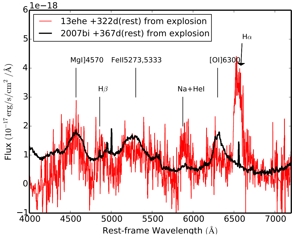
FIG. 7.— An optical nebular-phase spectrum of iPTF13ehe, taken +322days (rest-frame) from the estimated explosion date. We compare this spectrum with that of SN2007bi, which was taken at +367 days (rest-frame) from the estimated explosion date, downloaded from WISeREP (Gal-Yam et al. 2009; Yaron & Gal-Yam 2012).
