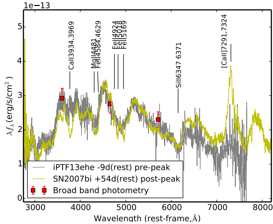
FIG. 4.— The optical spectrum during the photospheric phase of iPTF13ehe, taken at the pre-peak -9 days. We compare this spectrum with that of SN2007bi, which was proposed to be a PISN and powered by a large mass of ^{56}\text{Ni} (Gal-Yam et al. 2009).
