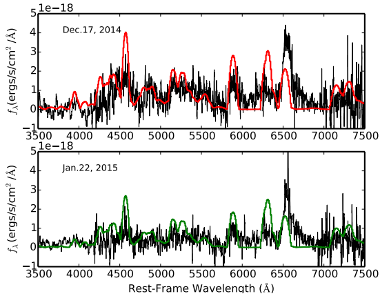
FIG. 9.— The 1-D nebular emission line models are plotted against the spectra taken on two different epochs separated by a month. The colored spectra are model predictions, and the black lines are observed spectra.
