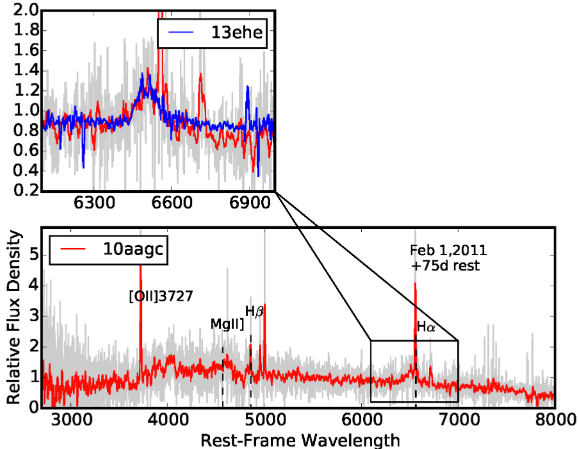
FIG. 10.— The late-time spectrum of PTF10aagc. We overlaid the smoothed spectrum (red line) on the top of the original data (grey line). The smoothing length is 13 pixels, corresponding to 15Å. In the zoom-in panel, we compare the broad H \alpha component from iPTF13ehe (blue line) to that from PTF10aagc (red line).
