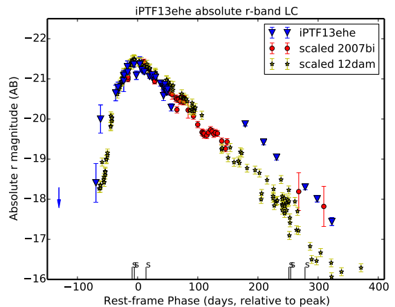
FIG. 2.— The iPTF13ehe rest-frame, k-corrected M_r light curve in comparison with those of SN2007bi and PTF12dam (Gal-Yam et al. 2009; Vreeswijk et al. 2015). The scaling factor is +0.1 magnitude for SN2007bi and 0.05 for PTF12dam.
