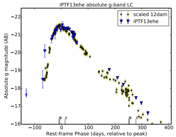
FIG. 3.— The Comparison of the iPTF13ehe M_g LC with that of PTF12dam (Vreeswijk et al. 2015). The PTF12dam g -band LC is shifted down by +0.15 magnitude.
