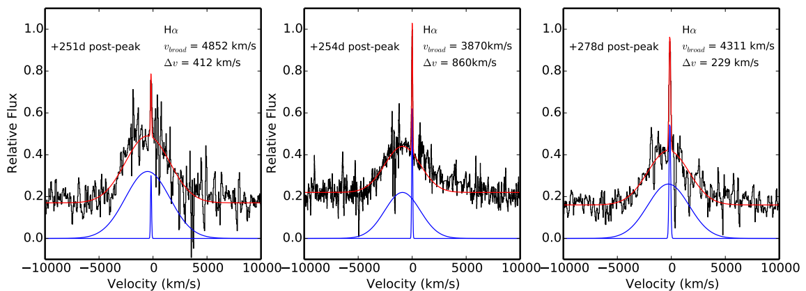
FIG. 8.— The Gaussian profile fitting to the broad and narrow H \alpha lines for the three epochs at +251, +254 and +278 days post-peak.
