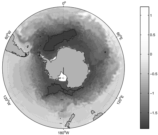
FIG. 1: Mean SSH (m) from ORCA025 model averaged over 1 January–29 February. Define regions A_{\text{Weddell,SSH}} = \{\text{SSH} < -1.75\text{m in Weddell Sea}\} and A_{\text{Ross,SSH}} = \{\text{SSH} < -1.6\text{m in Ross Sea}\} ; boundaries are shown dotted. The upper region is A_{\text{Weddell,SSH}} and the lower region is A_{\text{Ross,SSH}} .
