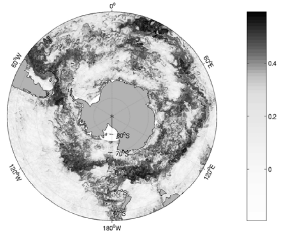
FIG. 3: Estimation of the finite-time Lyapunov exponent field from 1 January–29 February. Dark colors indicate regions of high stretching. The field was constructed using 100,213 boxes and 40 points per box; see [16].
