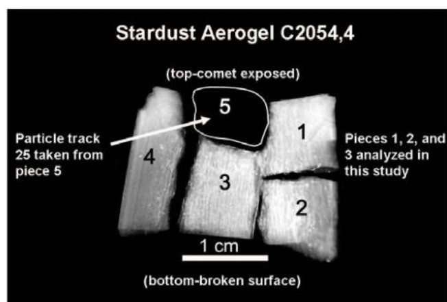
Fig. 1. The Stardust flight aerogel fragment C2054,4 sub-cutting diagram oriented with the comet exposed side at the top. Pieces 1, 2, and 3 were allocated during the preliminary examination period for LC-FD/ToF-MS analysis of amines at GSFC. Pieces 4 and 5 (which contained particle track 25) were not analyzed using this technique. Another comet-exposed aerogel sample C2086,1 that was not adjacent to a particle track was also analyzed (picture not shown). Aerogel photo courtesy D. Brownlee.
