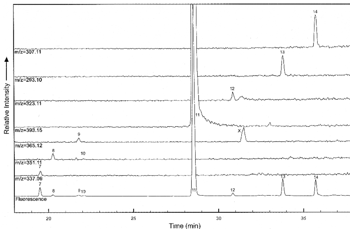
Fig. 5. LC-FD/ToF-MS chromatograms derived from the acid-hydrolyzed hot-water extract of comet-exposed aerogel sample C2054,4 show compounds detected by their fluorescence and mass. The peaks were identified by comparison of the retention time and exact molecular mass to those in the amine standard run on the same day. Only the exact mass traces corresponding to peaks detected in the fluorescence chromatogram were identified. See Table 1 for the identities of the numbered peaks.
