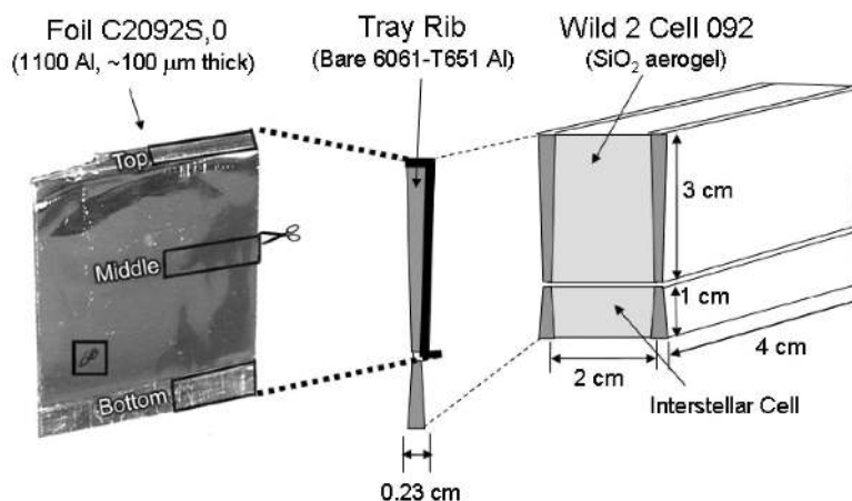
Fig. 2. The Stardust flight foil C2092S,0 showing the orientation of the foil in Wild 2 Cell 092 and the top, middle, and bottom pieces that were cut from the original foil and analyzed for amines separately. The top flap was directly exposed to Wild 2. The ink mark used to designate the aerogel contact side of the foil was removed prior to extraction of the remaining bulk foil sample. Another comet-exposed Stardust foil C2125N,2 was also analyzed in this study (picture not shown). Each foil was approximately 3 cm × 4 cm in size. Stardust collector tray rib and cell diagrams courtesy P. Tsou.
