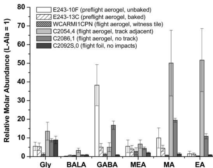
Fig. 4. A comparison of the relative molar abundances of glycine, \beta -alanine (BALA), \gamma -amino- n -butyric acid (GABA), ethanolamine (MEA), methylamine (MA), and ethylamine (EA) in the acid-hydrolyzed hot-water extracts of Stardust aerogel and foil. The abundances were normalized to L-alanine since this amino acid contaminant was found in all of the aerogel and foil samples. The uncertainties shown are based on the standard deviation of the average value of between two and eight separate measurements.
