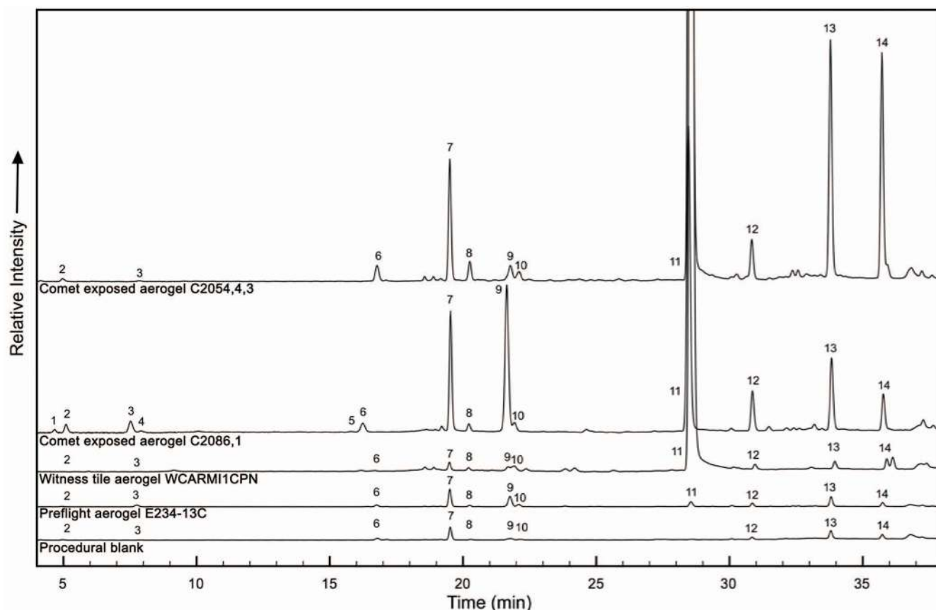
Fig. 3. LC-FD chromatograms showing OPA/NAC labeled primary amines from acid-hydrolyzed, hot-water extracts of the Stardust comet-exposed aerogel samples C2054,4,3 and C2086,1, the flight aerogel witness tile WCARM11CPN, preflight aerogel E234-13C, and a procedural blank. All major peaks were identified by retention time and positive electrospray ToF-MS collected simultaneously. There appear to be other minor peaks in these extracts, but their identities have not been established. Identifications for the numbered peaks are shown in Table 1.
