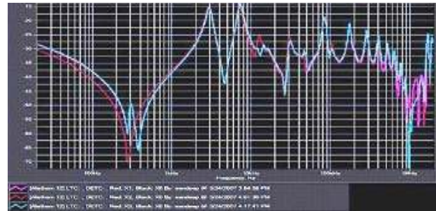
Figure 13 : LV winding response (HV open)
