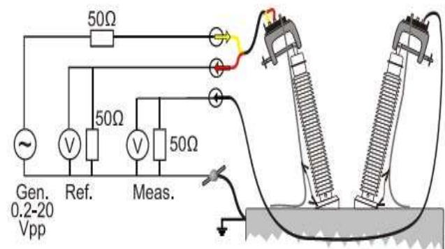
Figure 4 : SFRA Terminal Connection
