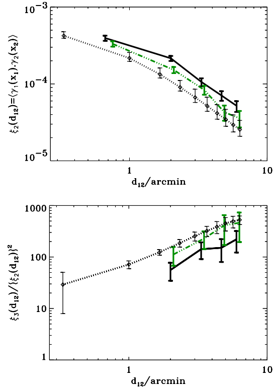
Fig. 3. Results for the VIRMOS-DESCART survey (similar to Fig. 1) compared to OCDM results (dotted lines) with cosmic variance computations.
