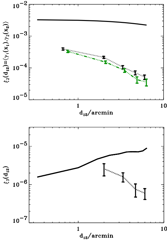
Fig. 2. Results for the VIRMOS-DESCART survey (dashed lines: when E and B mode contributions are included, dot-dashed line when B mode contributions are subtracted from the 2-point correlation function) compared the properties of the star anisotropy field statistics (solid lines).
