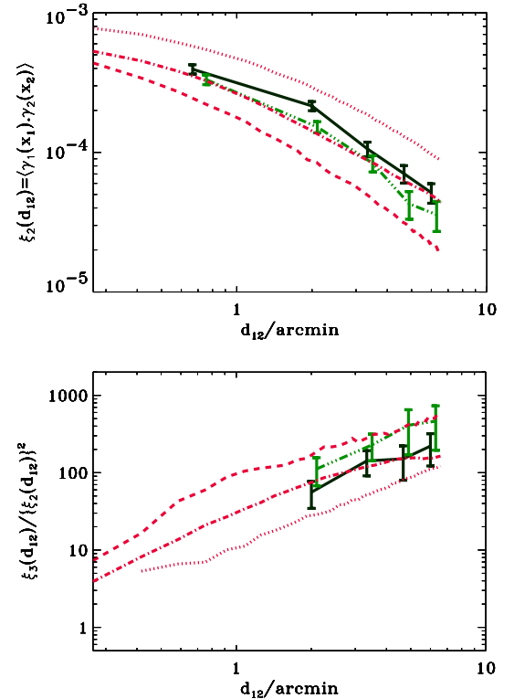
Fig. 1. Results for the VIRMOS-DESCART survey for the two point correlation function (top) and the reduced three point function (bottom). The solid line with error bars shows the raw results, when both the E and B contributions to the two-point correlation functions are included. The dot-dashed line with error bars corresponds to measurements where the contribution of the B mode has been subtracted out from the two-point correlation function (but not from \xi_3 there is no known way to do it). These measurements are compared to results obtained in \tau CDM, OCDM and \Lambda CDM simulations (dashed, dotted and dot-dashed lines respectively). ( \tau CDM, OCDM simulations are described in Jain et al. 2000; \Lambda CDM simulation was provided by M. White.)
