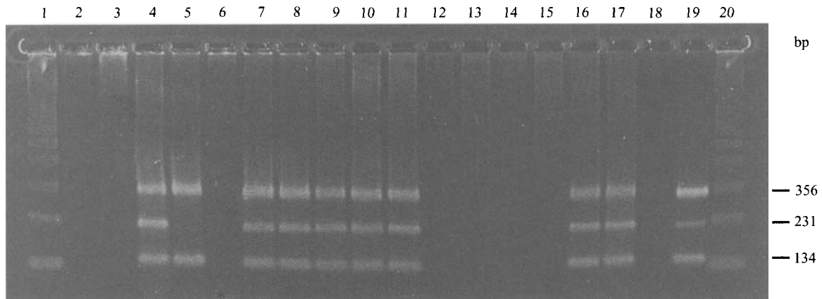
Fig. 1. Agarose gel electrophoresis of nucleic acid amplification products from Yersinia spp. using ail , virF and yst primers. Lanes 1 and 20, 123 bp DNA ladder (Bethesda Research Laboratories); Lane 2, Y. ruckeri ; Lane 3, Y. rohdei ; Lane 4, Y. enterocolitica O:1, 2, 3, human isolate (pyrazinamidase-positive); Lane 5, Y. enterocolitica O:3, human isolate; Lane 6, Y. enterocolitica O:5, lanes 7–10, Y. enterocolitica O:3, O:5, 27, O:5, 27, O:3, human isolates; Lane 11, Y. enterocolitica O:5, 27, porcine isolate; Lane 12, Y. bercovieri ; Lane 13, Y. frederiksenii ; Lane 14, Y. intermedia ; Lane 15, Y. mollaretii ; Lanes 16, 17, Y. enterocolitica O:3, human isolates; Lane 18, reagent control (no DNA); Lane 19, positive control, Y. enterocolitica O:13a, 13b.
