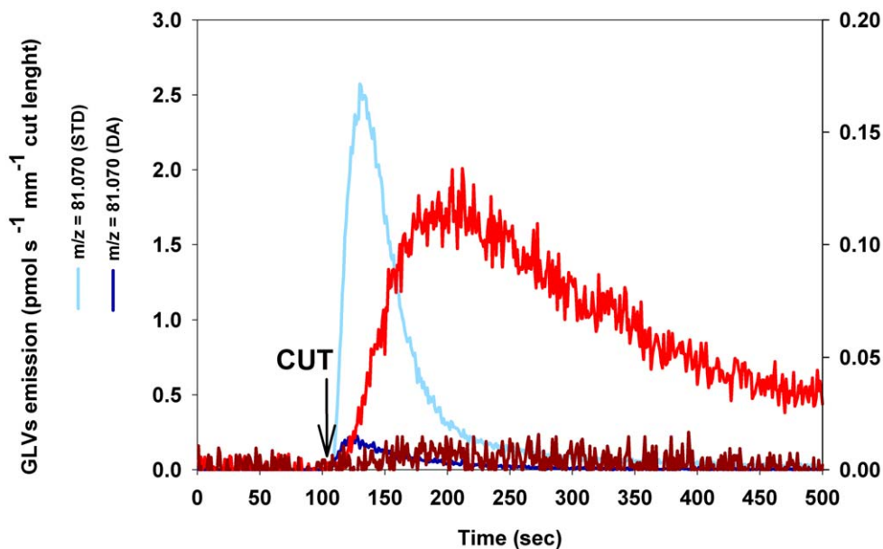
Figure 3. Release of GLVs after wounding Dactylis glomerata plants kept in dark conditions (24 hours/day) for 7 days long (DA) compared to Dactylis glomerata plants kept under standard circadian rhythm (12 hours light+12 hours dark) (STD). Different colors indicate different ions: m/z=81.070 [(Z)-3-hexenal+(E)-3-hexenal]; m/z=83.085 [(Z)-3-hexenol+(E)-3-hexenol+(E)-2-hexenol+hexanal]. Data shown are from a single leaf but are representative of experiments replicated four times on different leaves. doi:10.1371/journal.pone.0020419.g003
