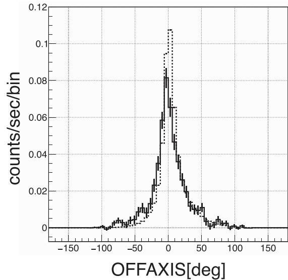
Fig. 9. Comparisons of the distributions of OFFAXIS events between the observation and the simulation. The solid line and the dotted line show the observation data and the simulation data, respectively.
