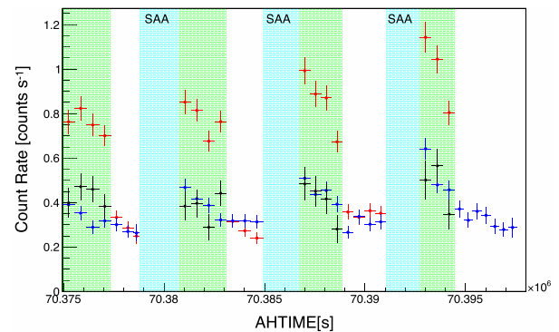
Fig. 3. Count rate of the SGD Compton camera as a function of time. The red and blue points show the count rates during the Crab observation and one day earlier. The black points show the count rates of the Crab GTI after subtracting the count rates one day earlier. The regions filled in green show the Crab GTI. The regions filled in cyan show time intervals excluded from the GTI due to the SAA passages. In the “white” portions of the time intervals, the Crab nebula was not able to be observed because of Earth occultation.
