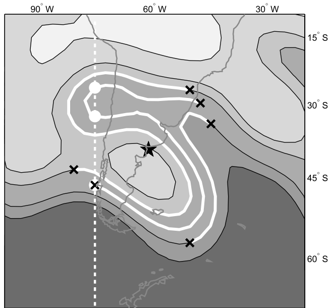
Figure 2. Detection of a wave breaking event on the 250 hPa absolute vorticity surface. The dashed white line denotes a meridian that intersects a contour at three overturning points which are denoted by closed white circles. The solid white contours connect all such overturning points. The black crosses denote each contour's west-most and east-most overturning points used to determine breaking orientation, and the black star denotes the centroid of the wave breaking event.
