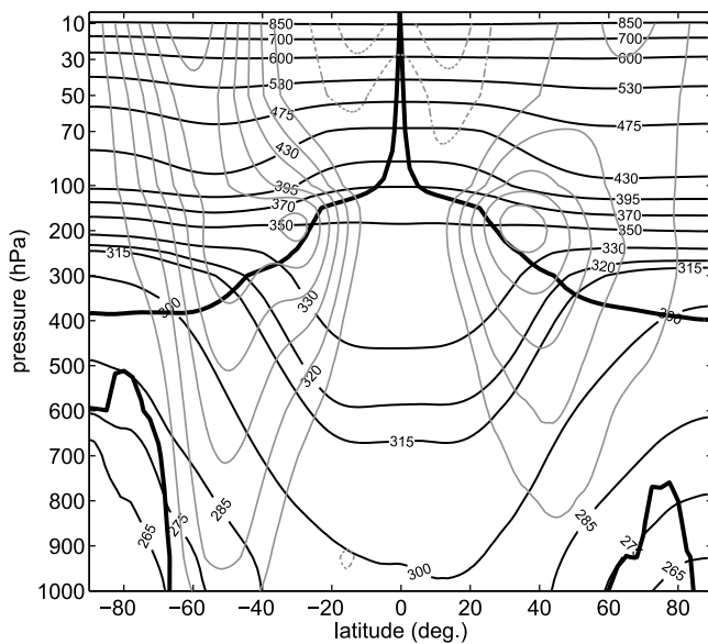
Figure 3. Annual-mean zonally averaged zonal winds (gray contours), potential temperature (labeled black contours) and the 2 PVU potential vorticity surface (thick black contour) from ERA-Interim Reanalysis. Dashed gray lines denote easterlies. The linear vertical spacing changes at 100 hPa to highlight the stratosphere.
