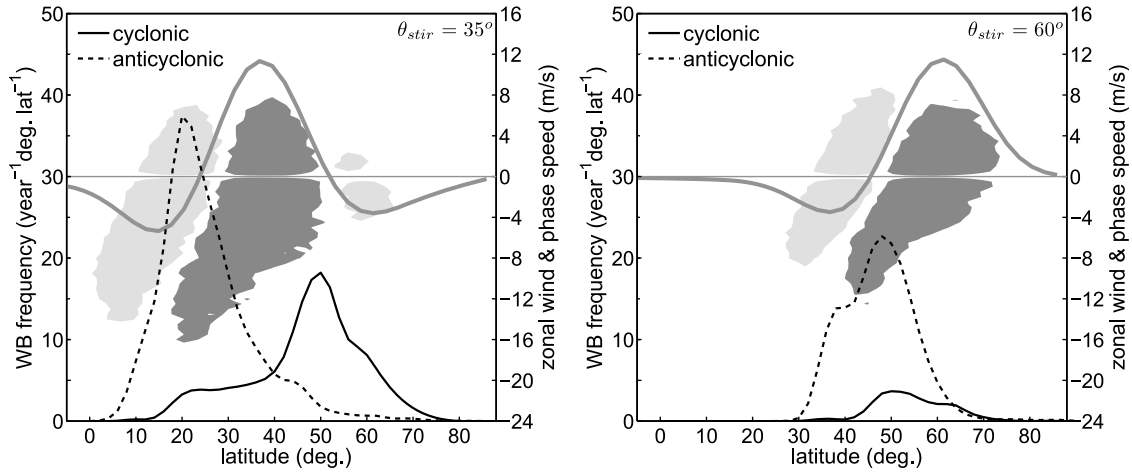
Figure 5. Shaded contours of \cos(\theta) \times D_\theta versus phase speed and latitude contoured at \pm 2 \times 10^{-7} \text{ m}\cdot\text{sec}^{-2} for \theta_{stir} = 35^\circ\text{N} and \theta_{stir} = 60^\circ\text{N} . Black dashed curves denote anticyclonic wave breaking frequency and black solid curves denote cyclonic wave breaking frequency. The gray curve denotes the zonal-mean zonal wind with axes on the right-hand-side of each panel.
