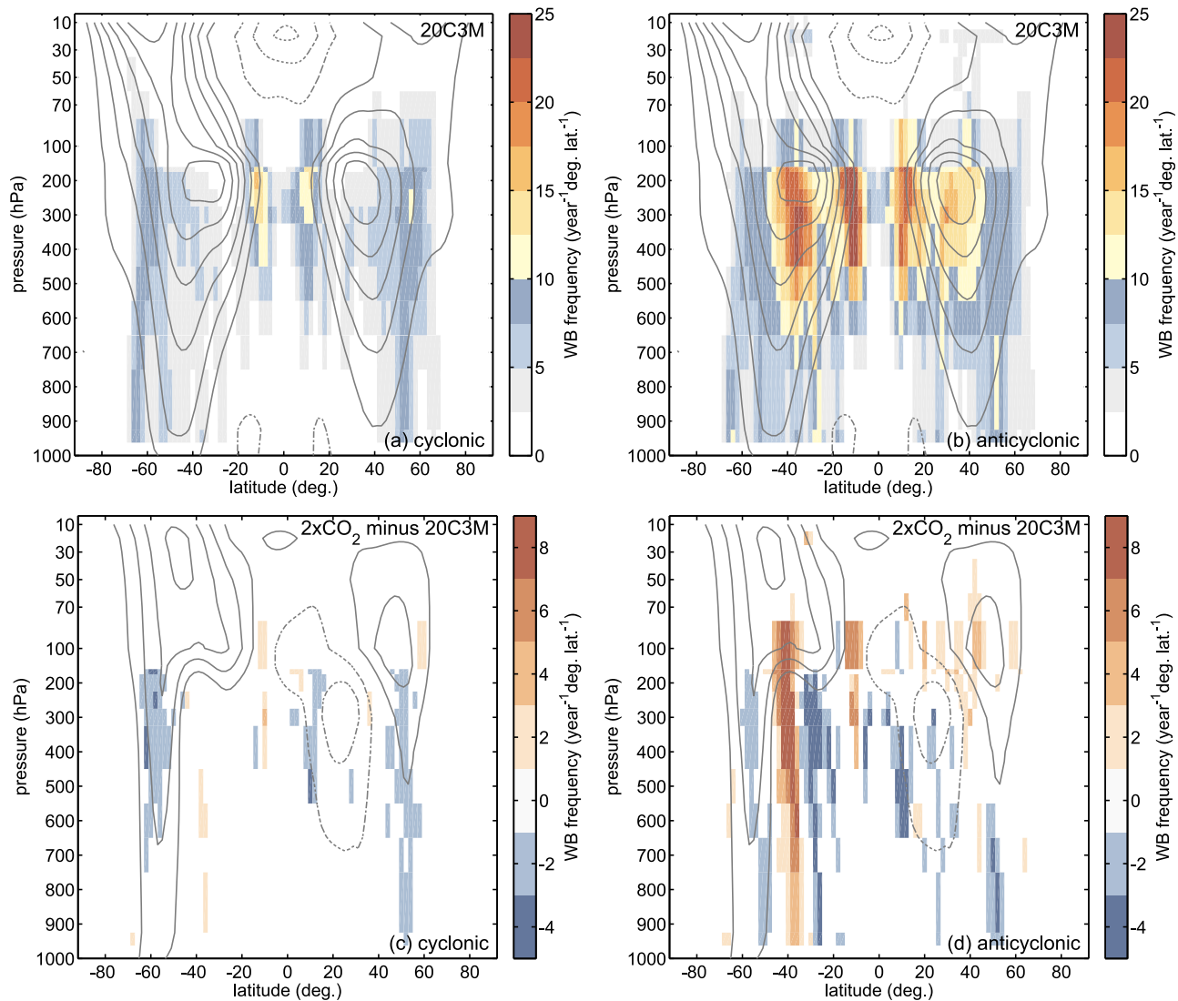
Figure 13. Zonally integrated wave breaking frequency for the GFDL CM2.0 model. (a) Cyclonic and (b) anticyclonic wave breaking frequency for the 20C3M (1961–2000) integration and (c, d) the difference in wave breaking frequency between the 2 \times \text{CO}_2 and 20C3M integrations, where only statistically significant changes are shaded (see Appendix A for details). Gray contours denote the zonal-mean zonal winds contoured every 5 m/s (Figures 13a and 13b), and change in the winds between the 2 \times \text{CO}_2 and 20C3M integrations contoured every 2 m/s with the zero lines omitted (Figures 13c and 13d). Dashed gray lines denote easterlies, and the linear vertical spacing changes at 100 hPa to highlight the stratosphere.
