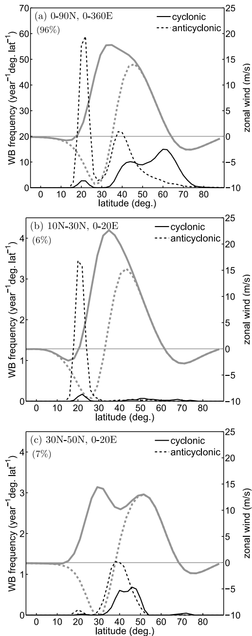
Figure 7. Wave breaking frequency versus latitude in the barotropic model for \theta_{stir} = 50^\circ\text{N} with a fixed subtropical jet centered at 30^\circ\text{N} . Frequencies are composited on days when there is a wave breaking event in (a) the hemisphere, (b) the sector 10^\circ\text{N} – 30^\circ\text{N} , 0^\circ – 20^\circ\text{E} , and (c) the sector 30^\circ\text{N} – 50^\circ\text{N} , 0^\circ – 20^\circ\text{E} . Black solid lines denote cyclonic wave breaking events and black dashed lines denote anticyclonic events. The gray solid curve denotes the total zonal-mean zonal wind in the specified sector composited on days when there is wave breaking there. The gray dashed curve denotes the eddy-driven component of the zonal winds. The percentage of days with wave breaking in the specified sector is shown in the upper-left-hand corner of each panel.
