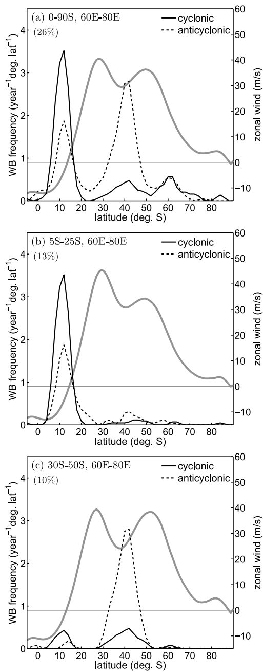
Figure 9. Wave breaking frequency versus latitude at 250 hPa from ERA-Interim during JJA. Frequencies are composited on days when there is a wave breaking event in the Indian Ocean sector ( 60^{\circ}\text{E} – 80^{\circ}\text{E} ) for various latitude bands. Black solid lines denote cyclonic wave breaking events and black dashed lines denote anticyclonic events. The gray solid curve denotes the total zonal-mean zonal wind in the specified sector composited on days when there is wave breaking there. The percentage of days within JJA with wave breaking in the specified sector is shown in the upper-left-hand corner of each panel.
