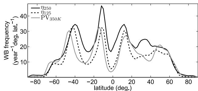
Figure 10. Meridional profiles of total wave breaking in ERA-Interim based on absolute vorticity on the 250 and 125 hPa surfaces ( \eta_{250} and \eta_{125} ) and potential vorticity on the 350 K potential temperature surface.
