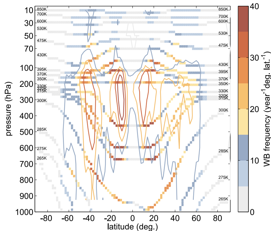
Figure 12. Annual mean, zonally integrated total wave breaking frequency for the ERA-Interim Reanalysis. Colored grid boxes denote frequencies calculated with isentropic potential vorticity and are plotted along their respective climatological potential temperature surfaces (see Figure 3). Contour lines denote wave breaking frequencies calculated using absolute vorticity on pressure surfaces.
