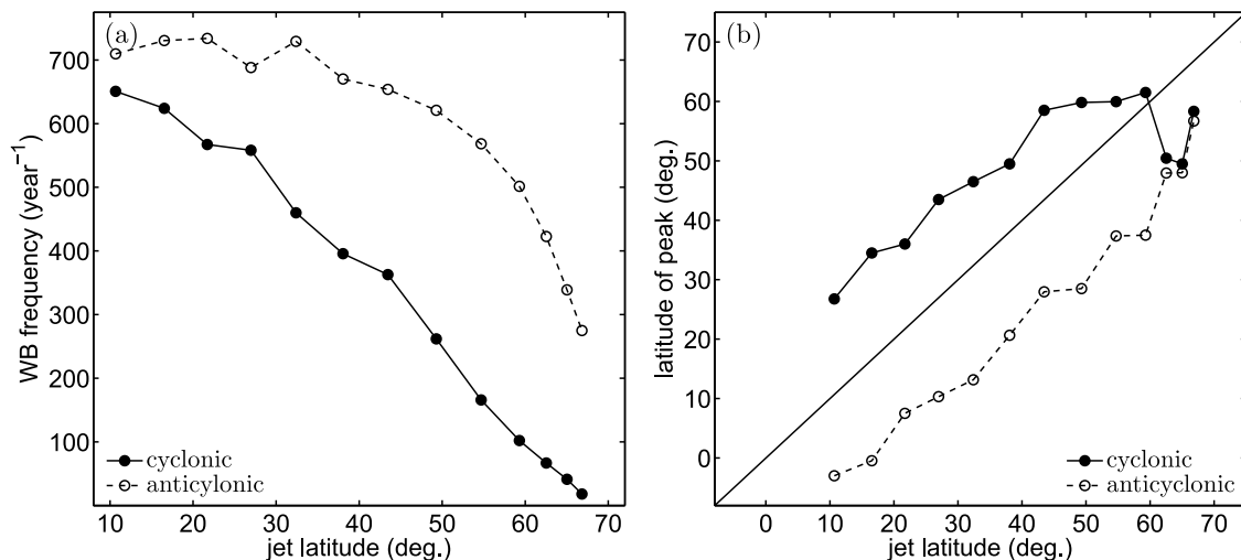
Figure 6. (a) Wave breaking frequency and (b) latitude of maximum wave breaking versus the latitude of the eddy-driven jet in the barotropic model separated into cyclonic and anticyclonic events (see text for note on classifications near the equator).
