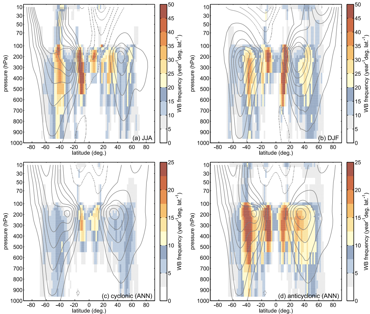
Figure 8. Zonally integrated wave breaking frequency for the ERA-Interim Reanalysis during (a) JJA and (b) DJF and in the annual-mean for (c) cyclonic and (d) anticyclonic orientations. Zonal-mean zonal winds are contoured every 5 m/s in gray, with the zero line omitted. Dashed gray lines denote easterlies, and the linear vertical spacing changes at 100 hPa to highlight the stratosphere.
