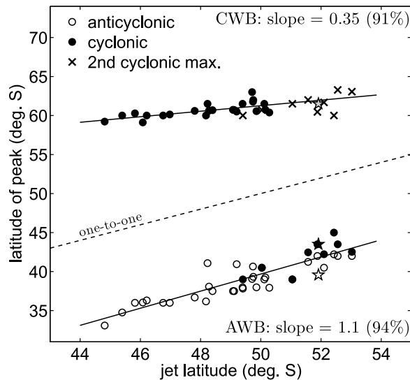
Figure 15. Latitude of maximum midlatitude wave breaking versus the latitude of the eddy-driven jet in the CMIP3 GCMs. Crosses denote the secondary maxima of cyclonic wave breaking when a double peaked distribution exists. ERA-Interim results are plotted as stars, with the gray star denoting the secondary cyclonic maximum. The solid lines denote the orthogonal-least squares fit for anticyclonic and the most poleward cyclonic wave breaking peaks, with the slope and percent variance explained displayed as text. The dashed line is the one-to-one line.
