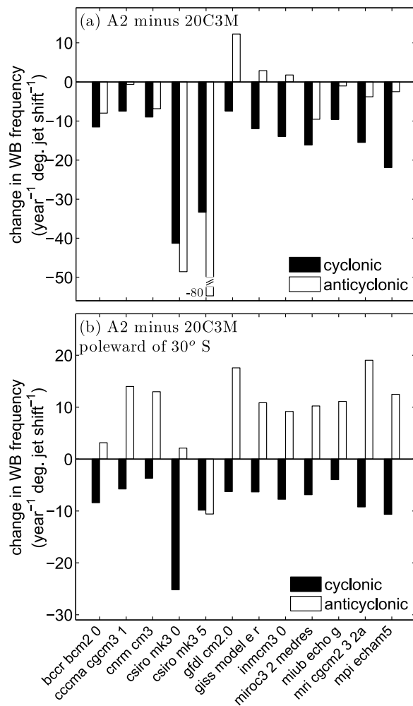
Figure 14. (a) Change in the number of Southern Hemisphere wave breaking events at 250 hPa per year per degree poleward shift of the jet between the A2 (2081–2100) and 20C3M (1961–2000) integrations for 12 CMIP3 GCMs. (b) Same as in Figure 14a except only for latitudes poleward of 30°S.
