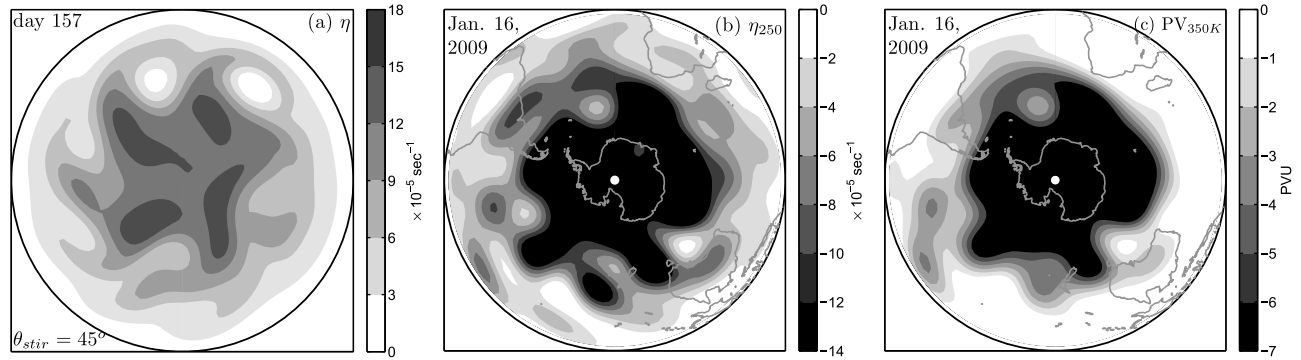
Figure 1. Snapshots of instantaneous fields of (a) absolute vorticity in the barotropic model, and ERA-Interim (b) 250 hPa absolute vorticity and (c) potential vorticity on the 350 K potential temperature surface. Figures 1b and 1c have been smoothed as outlined in Section 2.2.
