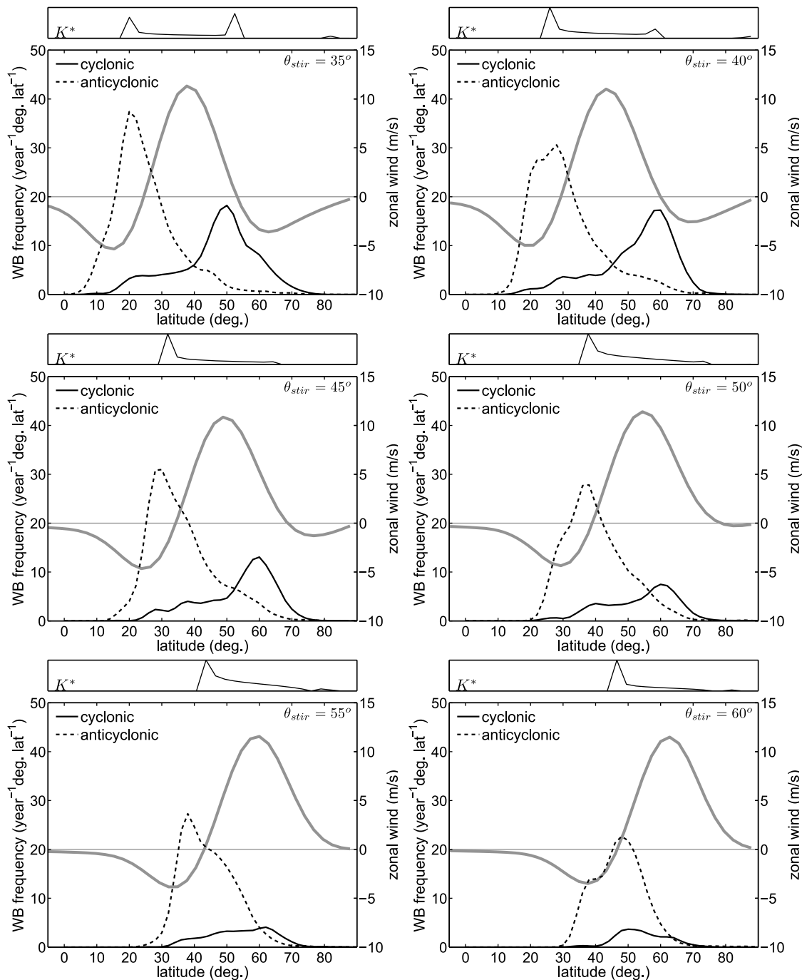
Figure 4. Wave breaking frequency versus latitude in the barotropic model where the stirring latitude is varied. Black solid lines denote cyclonic wave breaking events and black dashed lines denote anticyclonic events. The thick gray curve denotes the zonal-mean zonal wind with the axes on the right-hand side. K^* is plotted at the top of each panel for the power-weighted phase speed at the latitude of the jet.
