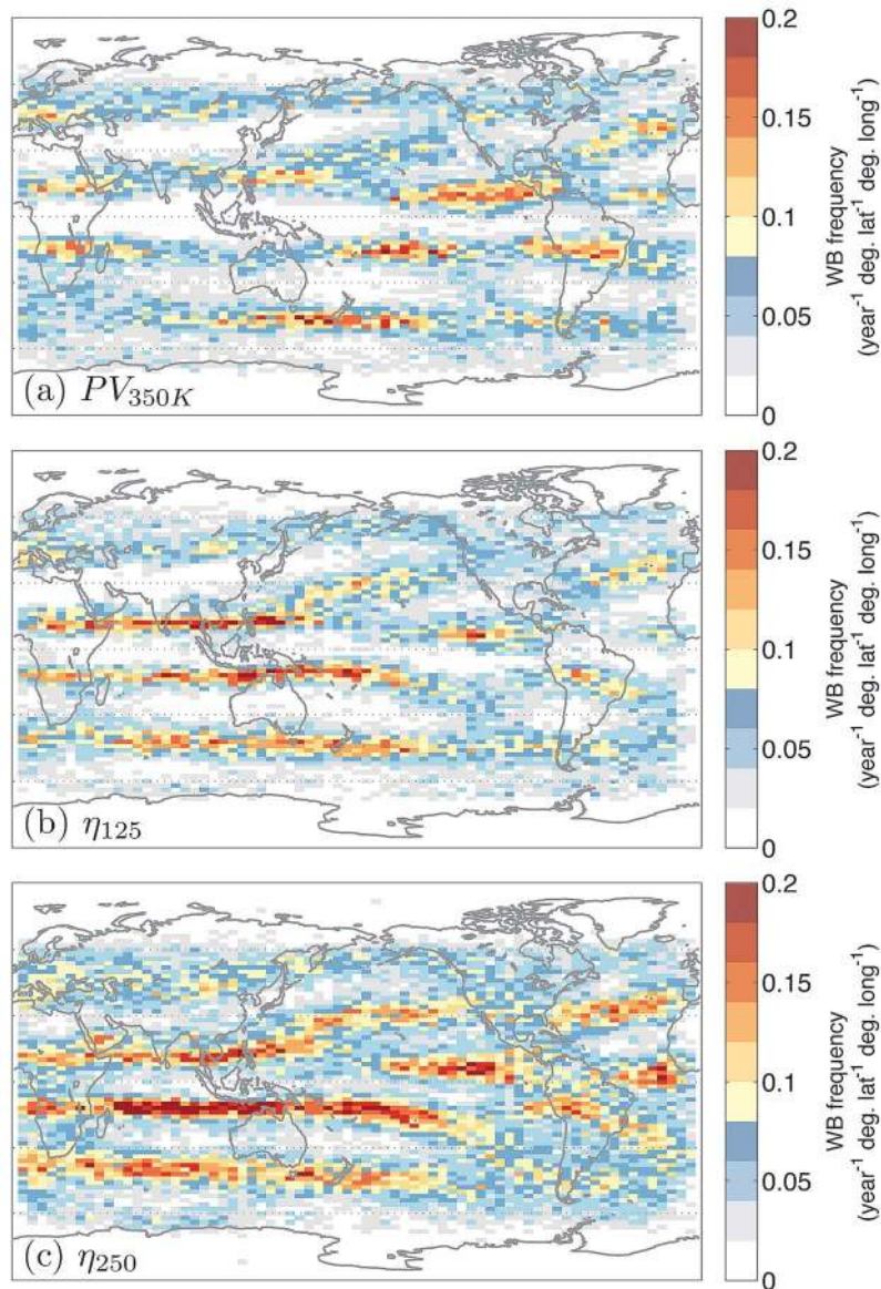
Figure 11. Latitude-longitude gridded wave breaking frequency in the annual mean from ERA-Interim based on (a) potential vorticity on the 350 K potential temperature surface, and absolute vorticity at (b) 125 hPa and (c) 250 hPa.
