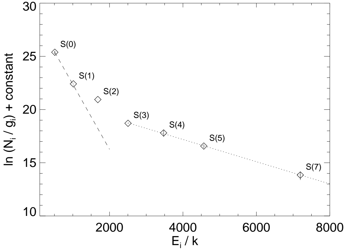
Fig. 3.— H_2 excitation diagram for NGC 6240, showing for the lines observed with the IRS, the upper level population divided by the level degeneracy, as a function of upper level energy. The lines have not been corrected for extinction. Errors are indicated as vertical bars for each line. The fits to the hot ( T \sim 957K ) and cold ( T \sim 164K ) components are indicated by a dotted and a dashed line, respectively.
