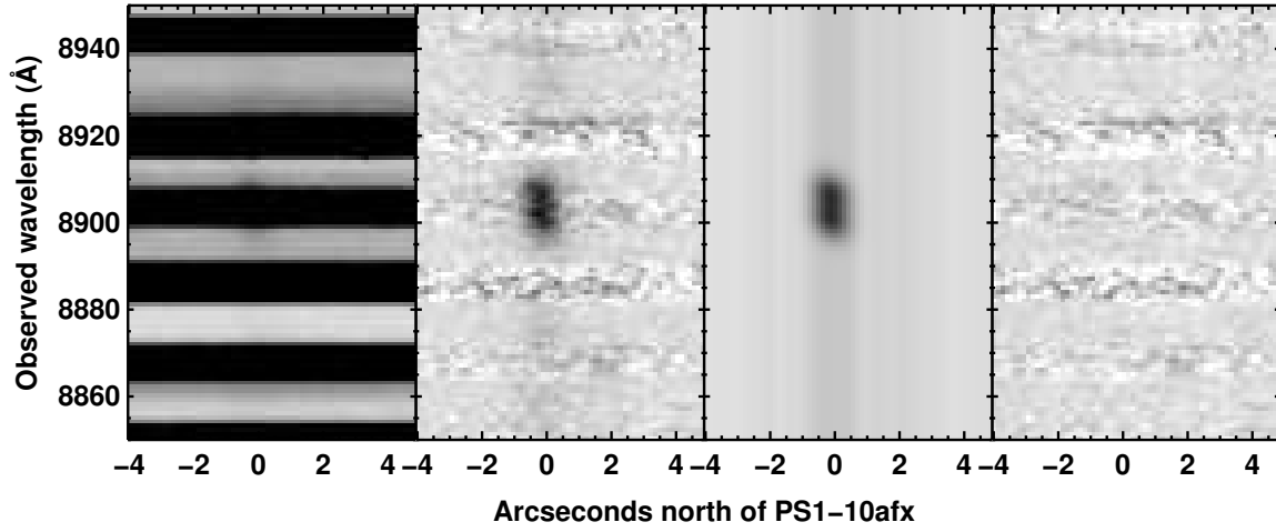
Figure S2: Composite 2-D spectra showing the [O II] emission from the host at z = 1.3885 . The first two panels on the left show the stacked spectra before and after removal of the sky background. The next panel shows the 2-D model for the emission lines and continuum, and the right panel shows the residual after this model was subtracted from the second panel.
