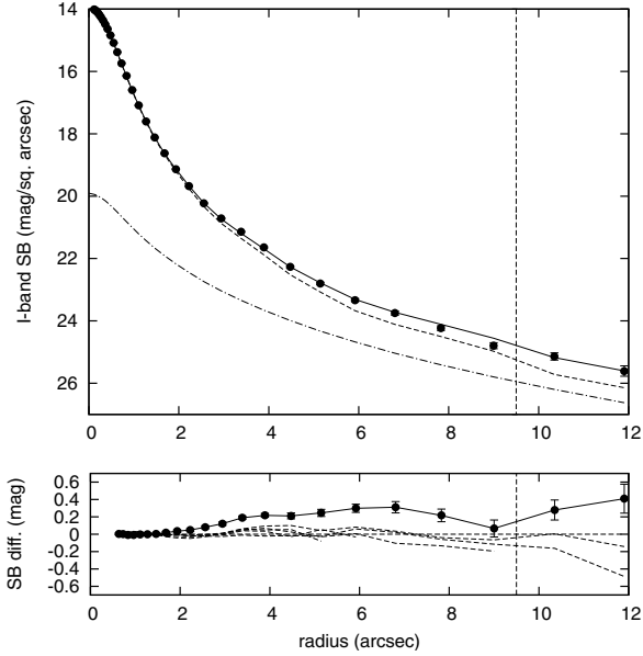
Fig. 2. Upper panel: the I -band surface brightness profile of S5 0716+714 (filled symbols). The solid line shows the core + host galaxy model, the dashed line the core component and the dot-dashed line the host galaxy component. The vertical dashed line shows the outer radius of the model-fitting region. Lower panel: the surface brightness profiles of S5 0716+714 (symbols and solid line) and stars 2, 3, 5, 6, S1, and S2 (dashed lines) relative to star 5. Each star is traced out to a radius at which the surface brightness can be determined to higher accuracy than 10%.
