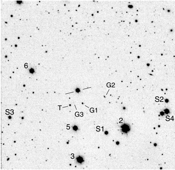
Fig. 1. The summed i -band image of S5 0716+714 obtained at the NOT in Dec. 22, 2007. The field size is 3.85 \times 3.7 arcmin, north is up and east is to the left. Object T is a transient or a very red object not visible in previous images of S5 0716+714, most of which were obtained in the R -band. The other labeled objects are discussed in the text.
