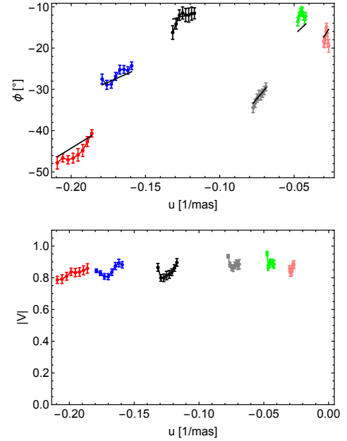
Fig. A.1. Example of a unary fit for a five-minute exposure on Sgr A* from April 22, 2019, 06:39:55. Top: phase \Phi as a function of projected baseline vector \mathbf{u} for the s-polarisation channel. Per baseline, eight spectral channels were included here. The black line is a unary model, which yields the offset from the interferometer pointing position to \Delta RA = 322 \pm 9 \mu\text{as} and \Delta Dec = 301 \pm 8 \mu\text{as} (formal fit errors). Bottom: the visibility modulus for the same data is constant and close to unity, consistent with the choice of fitting a single point source.
