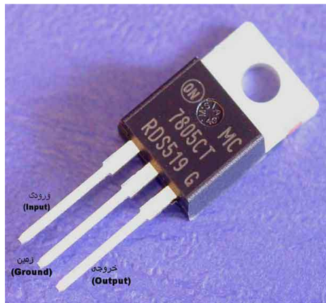
Figure 1: Voltage Regulator 7805
