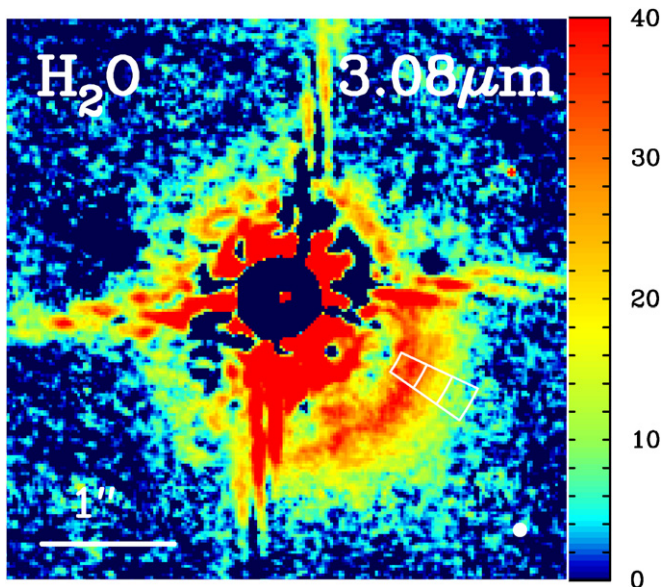
Figure 1. PSF-subtracted 3.08 \mu\text{m} image of the disk around HD 142527. The unit of intensity is \text{mJy arcsec}^{-2} . North is up; east is to the left. The occulting mask is 0''.6 . The spatial resolution is 0''.10 . The three enclosed regions (regions A, B, and C from inner to outer regions) on the southwest structure are the positions from which the spectra shown in Figure 3 are extracted.
