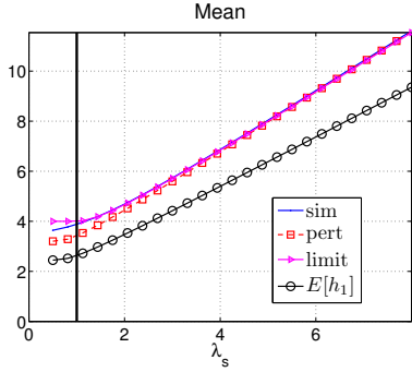
Fig. 1. Mean of \ell_1(E^{-1}H) vs. signal strength. The black vertical line is the limiting threshold for signal detection
