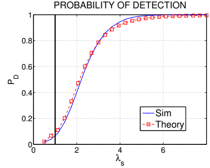
Fig. 3. Probability of detection at \alpha = 0.01 .
