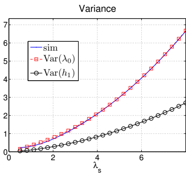
Fig. 2. Variance of \ell_1(E^{-1}H) vs. signal strength. Top two curves are comparison of simulation with Eq. (17).
