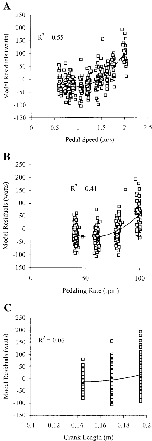
Fig. 2. Residuals of the mechanical power vs. metabolic cost regression model. Residuals were significantly related to pedal speed (A), pedaling rate (B), and crank length (C).
