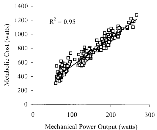
Fig. 1. Metabolic cost as a function of mechanical power. Mechanical power accounted for 95% of the variability in metabolic cost across the range of pedaling rates, pedal speeds, and crank lengths tested.
