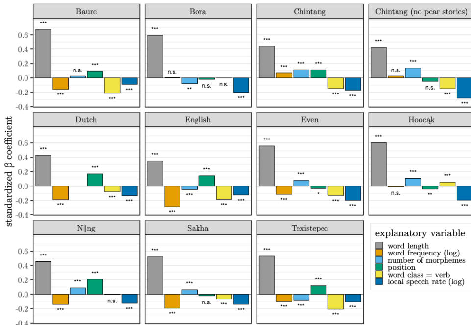
Figure 4. Comparison of standardized \beta coefficients for all six fixed effects in the mixed-effects models for the ten languages with significance stars based on likelihood ratio tests: n.s. p \geq 0.05 , * p < 0.05 , ** p < 0.01 , *** p < 0.001 .
