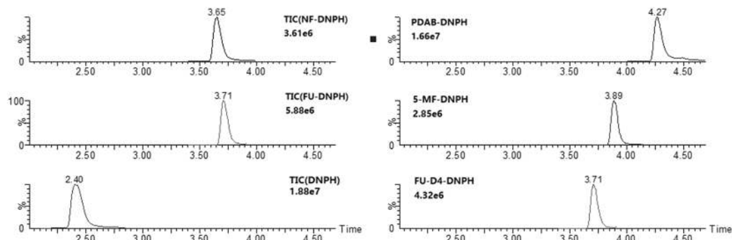
Figure 4. MRM chromatograms of DNP and five DNP derivatives at 10 µg/L.
