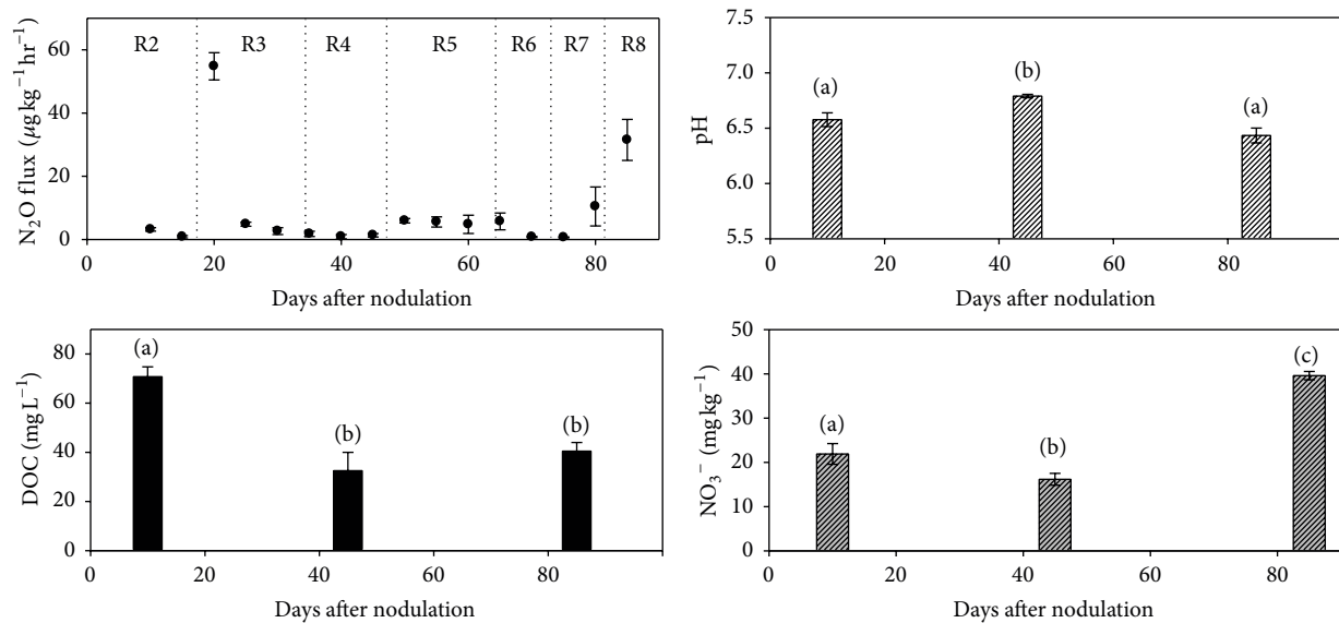
FIGURE 1: Temporal dynamics of N 2 O flux ( \mu\text{g kg}^{-1} \text{hr}^{-1} ), soil pH, DOC ( \text{mg L}^{-1} ), and NO 3 - -N ( \text{mg kg}^{-1} ) of IS treatment. Different lower case letters indicate a statistically significant difference at \alpha = 0.05 . R2: full flowering; R3: beginning pod; R4: full pod; R5: beginning seed; R6: full seed; R7: beginning of maturity; R8: full maturity. Means of 3 replicates with standard error.
